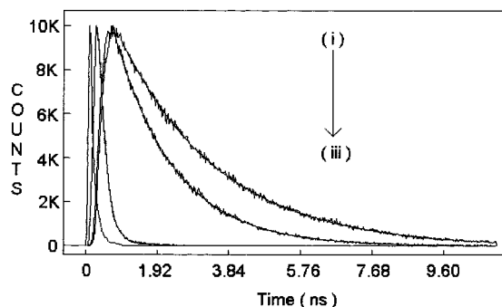
Figure 5. Fluorescence decays of merocyanine 540 in (i) 0.09 M AOT/ n -heptane/ H_2O , w_0 = 4 , (ii) 0.09 M AOT/ n -heptane/ H_2O , w_0 = 32 , and (iii) water.
