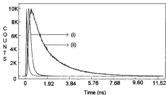
Figure 6. Fluorescence decays of merocyanine 540 in (i) water and (ii) 360 \mu M buffered aqueous solution of BSA.
