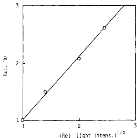
Figure 10. Relative R_p vs. (\text{rel. light intens.})^{1/2} for the photopolymerization of MMA with BPC- \text{CCl}_4 system in dichloromethane.
