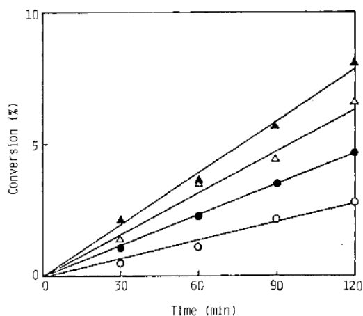
Figure 9. Effect of light intensity on the photopolymerization of MMA with BPC- \text{CCl}_4 system in dichloromethane: MMA, 5\text{ cm}^3 ; \text{CH}_2\text{Cl}_2 , 4\text{ cm}^3 ; PBC, 1 \times 10^{-3}\text{ mol dm}^{-3} ; temp, 303 K; relative light intensity, \circ , 1; \bullet , 2; \triangle , 4; \blacktriangle , 6.
