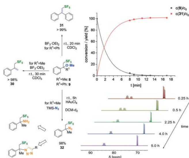
Figure 4. Top: Elimination of the methoxy substituent of 8 and 9 by 10.0 equiv \text{BF}_3 \cdot \text{Et}_2\text{O} , and representative ^{19}\text{F} -NMR kinetics for the conversion of 9 to 31 . Bottom: Azidation of 8 to 32 (with potential following chemistry) and time-resolved ^{19}\text{F} -NMR spectroscopy analysis for the conversion of 8 into 32 .
