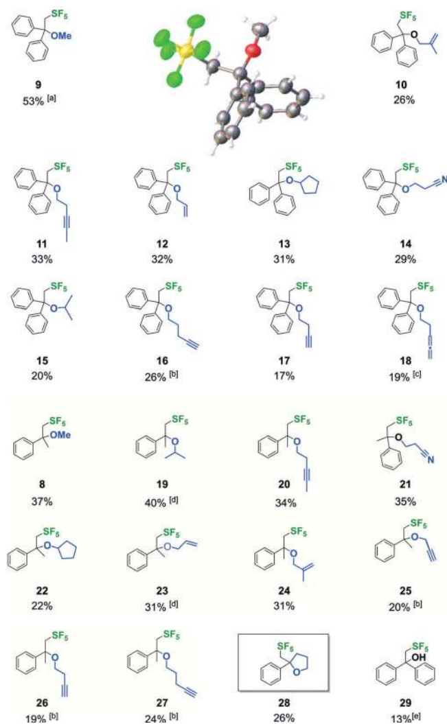
Figure 3. Substrate scope for the for the pentafluorosulfanylation of 1 and 2 and XRD structure of product 9 . Yields were determined by ^{19}\text{F} -NMR spectroscopy in the crude reaction mixture. General reaction conditions: 0.20 mmol, 0.20 M in MeCN, 10 mol% 3 , 10 mol% \text{BF}_3 , 22 h, 20°C, 2.8 bar (15 equiv) \text{SF}_6 , 368 nm. [a] Yield determined by GC-FID, 20 mol% \text{BF}_3 used. [b] 3.0 equiv alkynol. [c] 0.15 M, 14 equiv. allene. [d] 1.00 mmol scale. [e] Prepared with 1-ethynyl-1-cyclopentanol.
