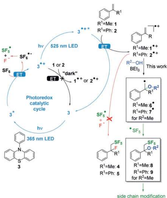
Figure 2. Proposed mechanism of photoredox catalytic activation of \text{SF}_6 by N-phenylphenothiazine ( 3 ) for pentafluorosulfanylation of \alpha -methyl ( 1 ) and \alpha -phenyl ( 2 ) styrenes, and addition by fluoride as an internal nucleophile to give 4 and 5 or alcohols ( \text{R}^2\text{-OH} ) as external nucleophiles to give products 8 and 9 (shown for \text{R}^2 = \text{Me} ).
