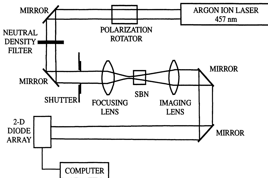
Figure 4. Experimental Apparatus
