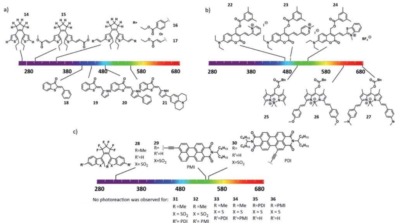
Fig. 11 Extension of the \pi -conjugation as a method to red-shift the activation wavelength of molecular photoswitches (a and c) and photocages (b).
