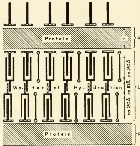
FIG. 46.—Hypothetical structure of chloroplasts according to Hubert. Rectangular hatched bars represent hydrophilic groups, black bars—lipophilic groups; combination of the two at right angles—chlorophyll molecules. The dumbbell-shaped structures represent carotenoid molecules. Phospholipide molecules are indicated by the black magnet-shaped structure attached to a hatched "handle."
