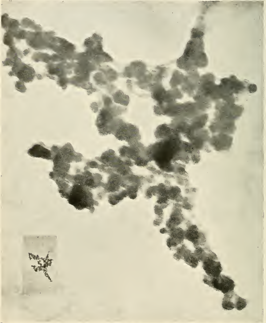
FIG. 43.—Portion of a chloroplast of Elodea canadensis , showing units (after Roberts 1942 2 ). * Inset, \times 10,000 ; main figure, \times 100,000 .
