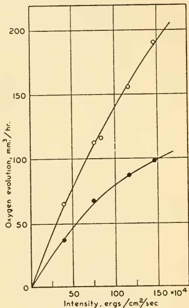
FIG. 31.—Light curves of photosynthesis in Chlorella with and without ethylurethan (after Wassink, Vermeulen, Reman, and Katz 1938). \circ : not inhibited; \bullet : inhibited by 0.05 ml. 50% urethan in ml.
