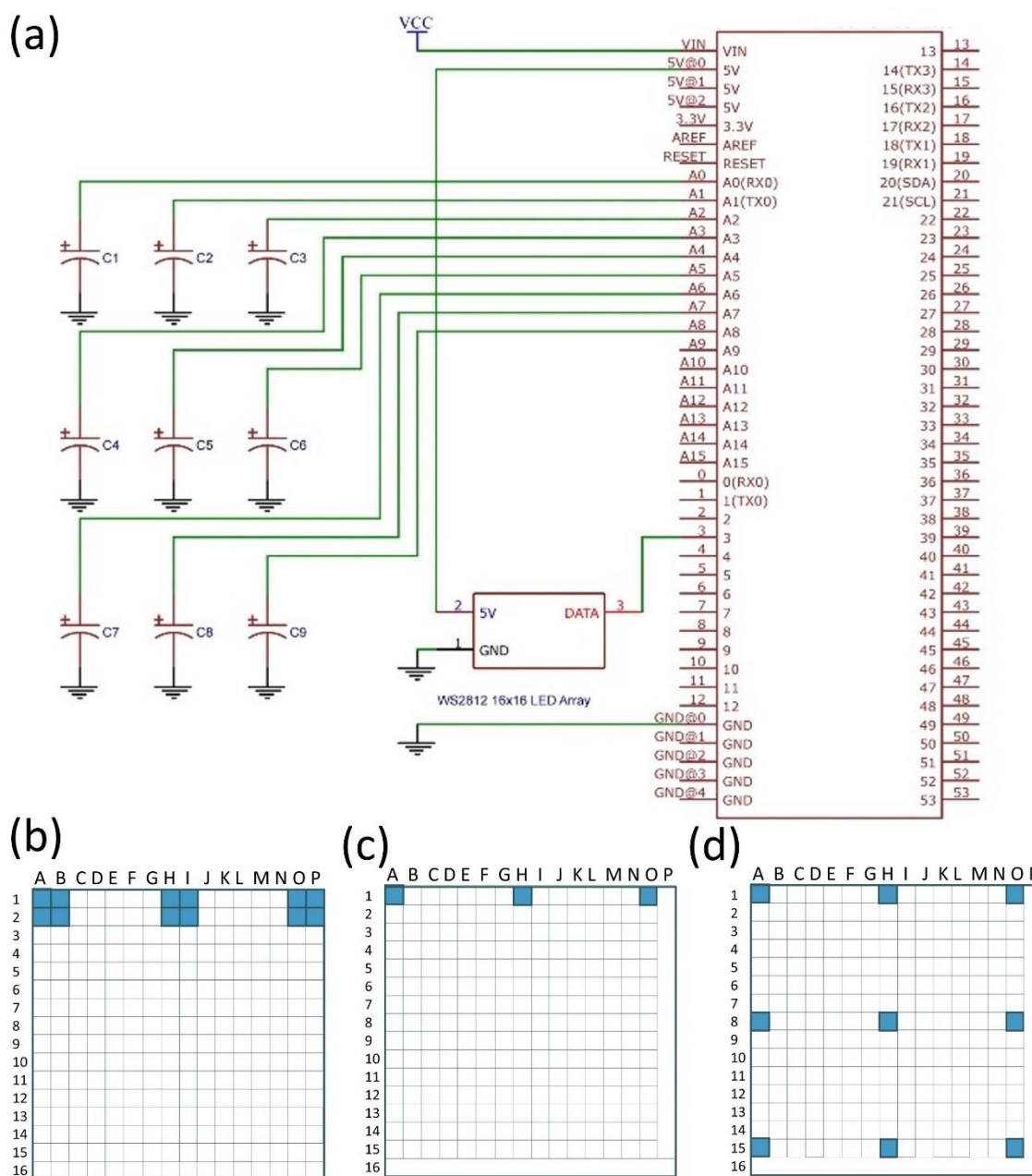
Figure S3. Electronic interface used to translate voltage signals from the a 9-pixel touch sensor to an LED array. a) Each pixel in the 9-pixel device is represented by an electrochemical capacitor (C1 to C9). The Au electrodes of each of the nine pixels are connected to analog input pins A0-A8 on a microcontroller board and the ITO electrodes are connected to ground. The microcontroller's on-board analog-to-digital converter read in the voltages from each pixel and the data are recorded. A 5-volt WS2812 16-by-16 multicolour LED array panel was also connected to the microcontroller. b) In the case of touch registering using a 3-pixel device, the signal from each pixel is translated to a block of four LEDs in the 16-by-16 array. Each LED in the array is identified by its column letter (A to P) followed by row number (1 to 16). Pixel 1 in the sensor corresponds to A1-B1-A2-B2, pixel 2 to H1-I1-H2-I2, pixel 3 to O1-P1-O2-P2. c) In touch-tracing in the 3-pixel device, pixel 1 corresponds to A1, pixel 2 to H1 and pixel 3 to O1. d) For touch-tracing in the 9-pixel device, the signals from pixels 1 to 9 is translated to
