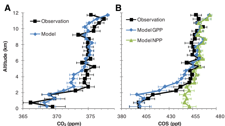
Fig. 1. Vertical profiles of COS and \text{CO}_2 along INTEX-NA flight paths. Mean concentrations for all continental INTEX-NA data for \text{CO}_2 (A) and COS (B) (error bars indicate \pm 95\% CI, n = 70 average observations in each bin). Model results were interpolated to time and location of each observation. ppm, parts per million.
