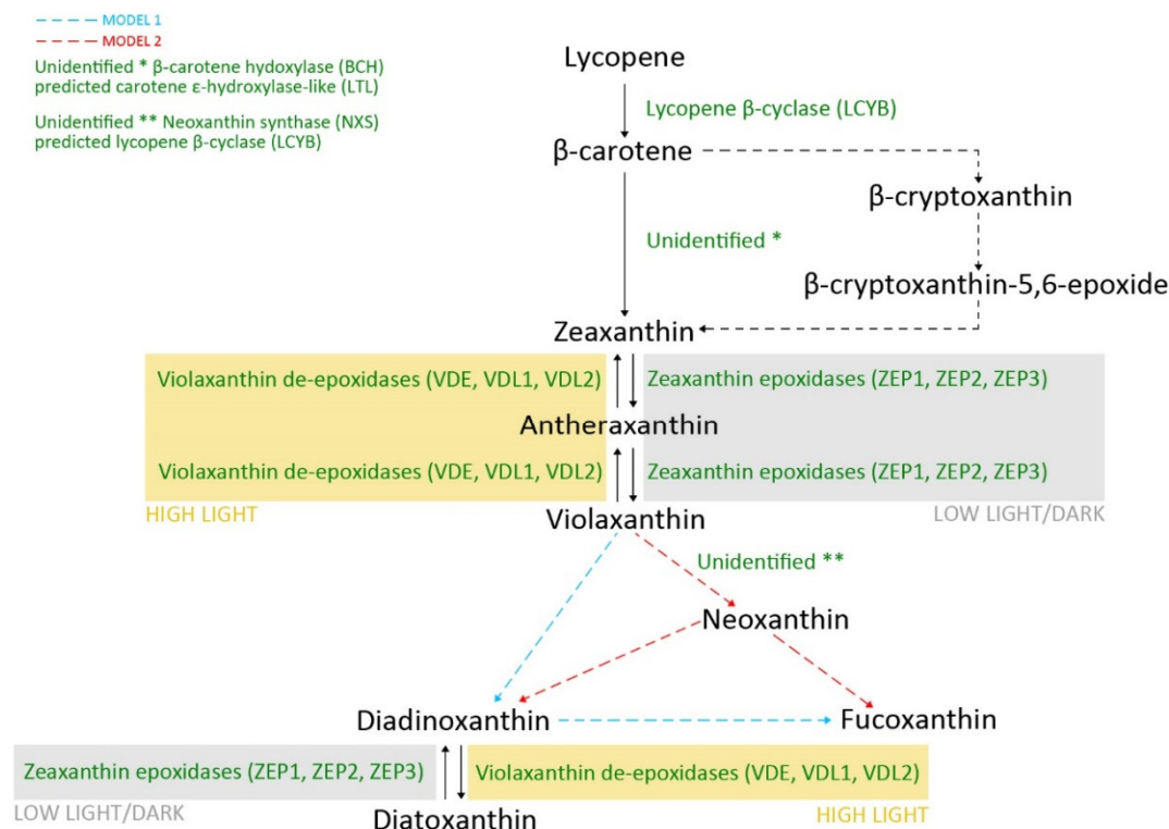
Figure 2. Biosynthetic pathway of photosynthetic carotenoids in the diatom Phaeodactylum tricornutum from lycopene to fucoxanthin and diatoxanthin.
