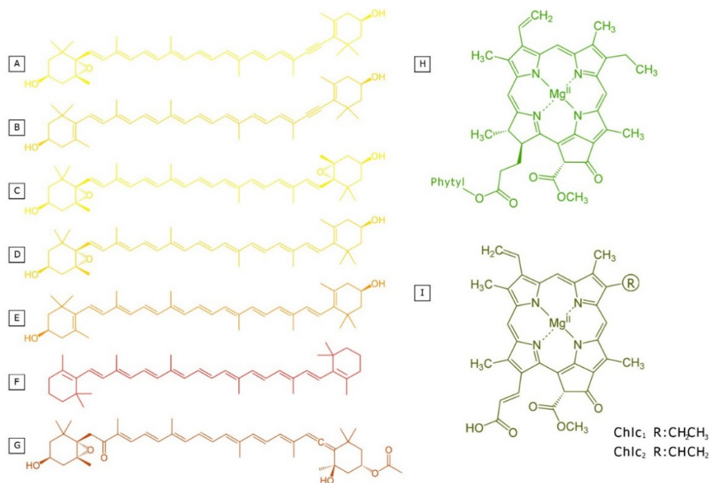
Figure 1. Structural formula of photosynthetic pigments in diatoms including all-trans carotenoids: (A) diadinoxanthin; (B) diatoxanthin; (C) violaxanthin; (D) antheraxanthin; (E) zeaxanthin; (F) \beta -carotene; (G) fucoxanthin; and chlorophylls: (H) chlorophyll a ; (I) chlorophyll c .
