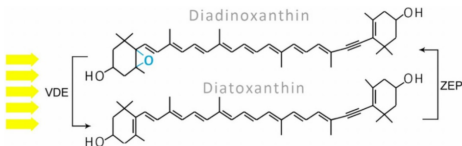
Figure 5. The diadinoxanthin cycle: in high light, diadinoxanthin with one epoxy group is converted to epoxy-free diatoxanthin by violaxanthin de-epoxidase (VDE); the reverse reaction is observed in low light and dark and is catalyzed by zeaxanthin epoxidase (ZEP).
