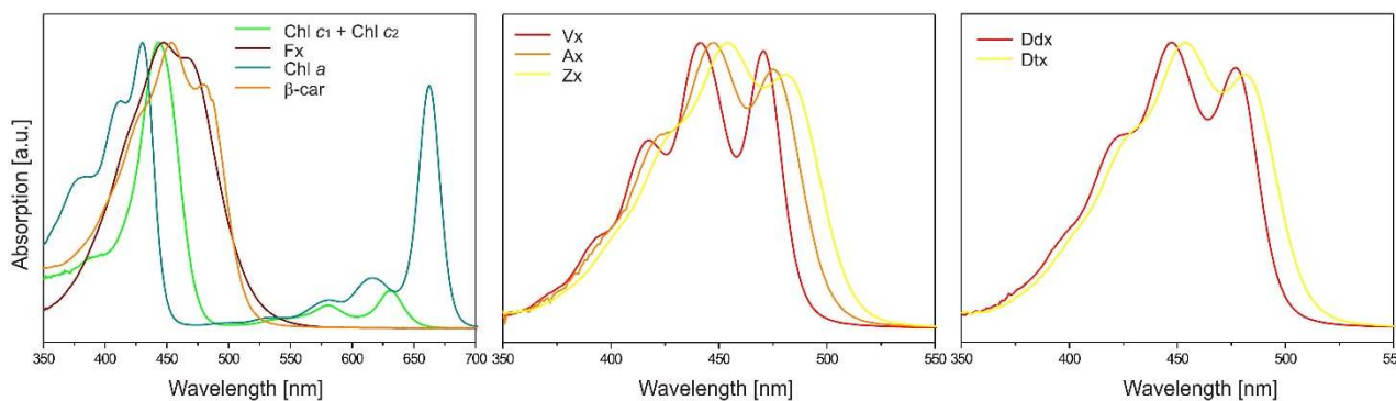
Figure 8. Absorption spectra of photosynthetic pigments recorded during HPLC-DAD analysis performed on extracts from the diatom P. tricornutum with the method by Kraay and co-workers [118]. The spectra were normalized at \lambda_{\text{max}} .
