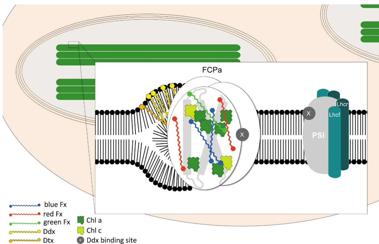
Figure 3. Simplified model of diatom thylakoid membrane showing the localization of photosynthetic pigments within FCP, PS I, and those localized within an monogalactosyldiacylglycerol (MGDG) shield surrounding the FCP. See the text for more information. Based on Gundermann and Büchel [60].
