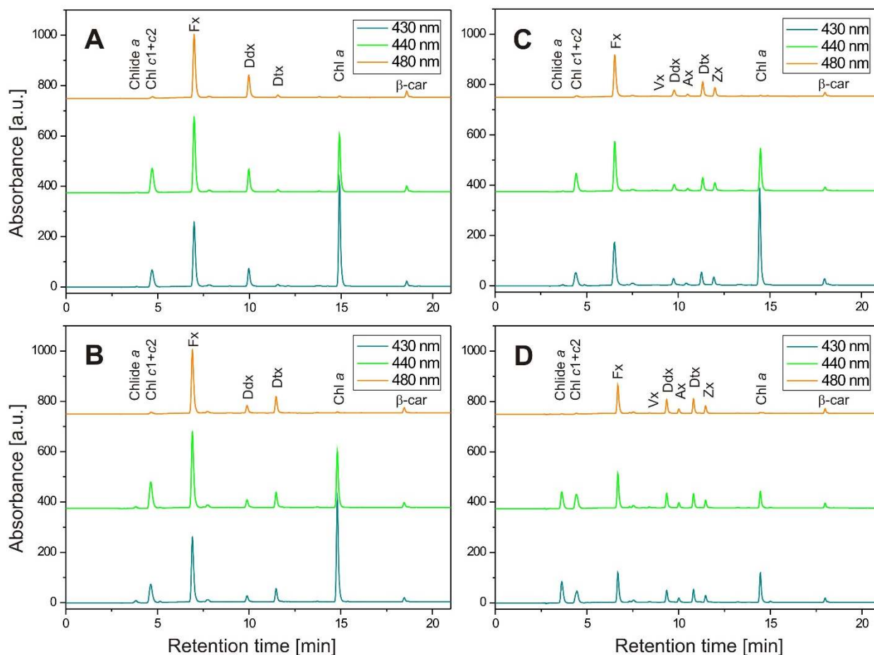
Figure 7. Examples of HPLC chromatograms of absorbance recorded at 430, 440, and 480 nm obtained with the method by Kraay and co-workers [117] for pigment extracts from the diatom P. tricornutum : (A) 1 h dark incubated cells growing in LL; (B) 1 h HL illuminated cells growing in LL; (C) 1 h HL illuminated cells growing in ML; (D) 48 h HL illuminated cells growing in LL. LL: white light with the intensity of 100 \mu\text{mol m}^{-2}\cdot\text{s}^{-1} in a 16 h light/8 h dark photoperiod; ML: white light with the intensity of 700 \mu\text{mol m}^{-2}\cdot\text{s}^{-1} in a 6 h light/18 h dark photoperiod; HL: white light with the intensity of 1250 \mu\text{mol m}^{-2}\cdot\text{s}^{-1} .
