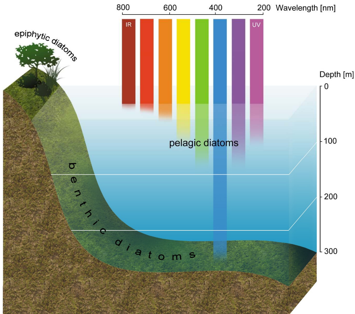
Figure 4. Spectra composition of light depending on the depth.
