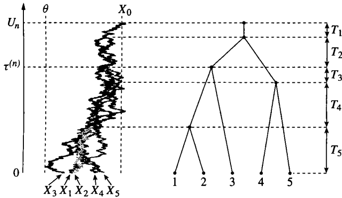
FIGURE 1: Left : A branching Ornstein–Uhlenbeck process simulated on a realization of the Yule n -tree with n = 5 tips using the TreeSim [38], [39] and mvSLOUCH [7] for packages R [32]. Parameters used are \alpha = 1 , \sigma = 1 , X_0 - \theta = 2 , after the tree height U_n was scaled to 1. Right : The species tree disregarding the trait values supplied with the notation for the interspeciation times. For the pair of tips (2,3) the time \tau^{(n)} to their most recent common ancestor is marked on the time axis (starting at present and going back to the time of origin).
