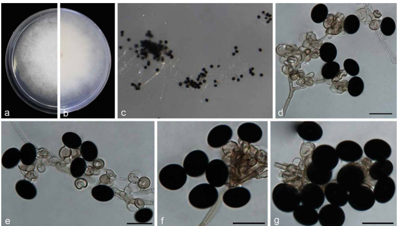
Fig. 11 Nigrospora lacticolon (from ex-type strain CGMCC3.18123). a–b. Upper surface and reverse overview of culture 6 d after inoculation on PDA medium; c. colony on SNA; d–f. conidiogenous cells giving rise to conidia; g. conidia. — Scale bars = 10 \mu m.
