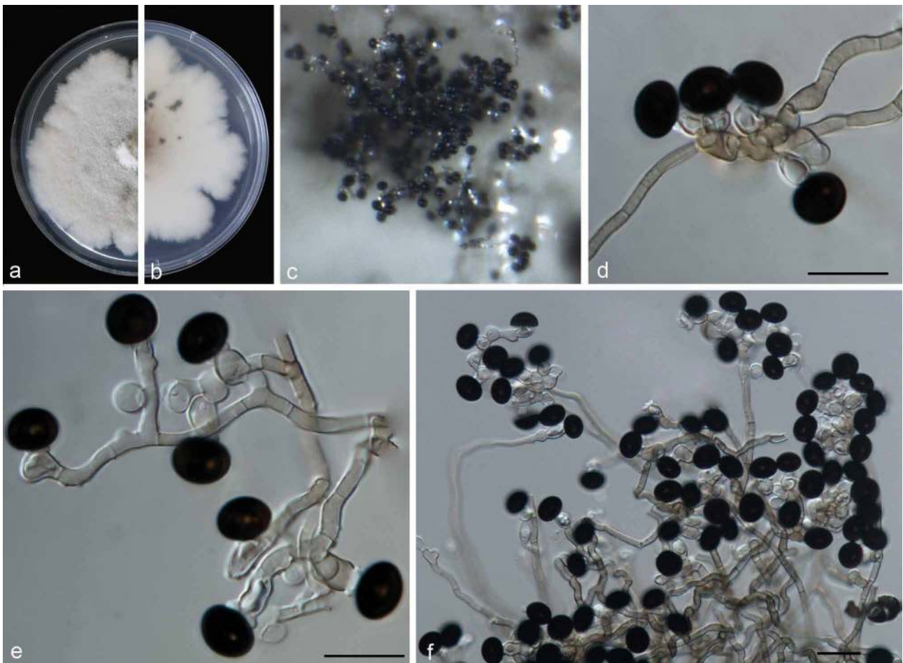
Fig. 9 Nigrospora guilinis (from ex-type strain CGMCC3.18124). a–b. Upper surface and reverse overview of culture 9 d after inoculation on PDA medium; c. colony on SNA; d–e. conidiogenous cells giving rise to conidia; f. conidia. — Scale bars: d–e = 10 \mu m; f = 20 \mu m.
