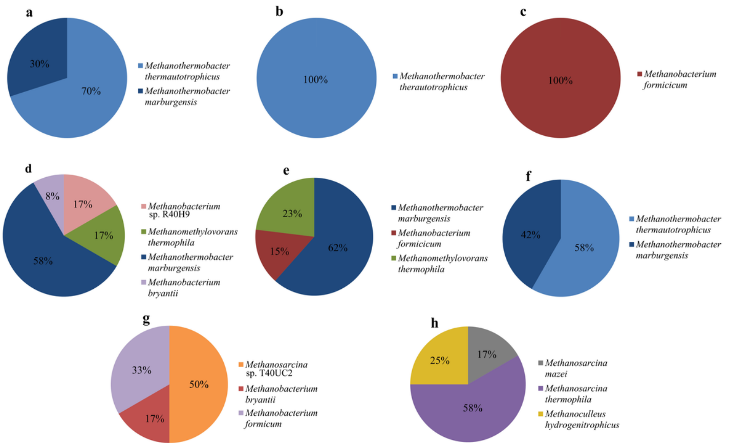
Figure 2 Pie charts describing the diversity, distribution and abundance of various methanogenic species in Chumathang (a), Puga (b), Unkeshwar (c), Rajawadi (d), Tural (e), Unhavare (f), Chopda 1 (g) and Chopda 2 (h) hot spring
