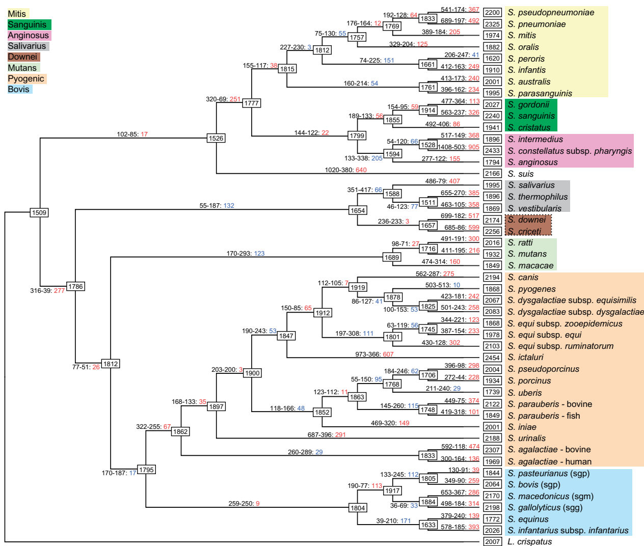
Fig. 2. —Result of gene gain/loss analysis. Boxes on nodes and tips of the phylogeny show genome size (genome size calculations exclude one MCL gene cluster that was excluded from the analysis—see Materials and Methods). Numbers on branches show the number of gains, losses, and the overall balance (gain-loss: balance), with red indicating an overall gain and blue an overall loss. Color shading for each major Streptococcus group follows figure 1.
