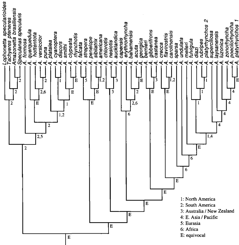
FIG. 2. Biogeographic reconstruction of ancestral areas using Ronquist's (1997) method of dispersal-vicariance analysis. Subspecies are combined and the weighted molecular (Fig. 1) topology is shown.
