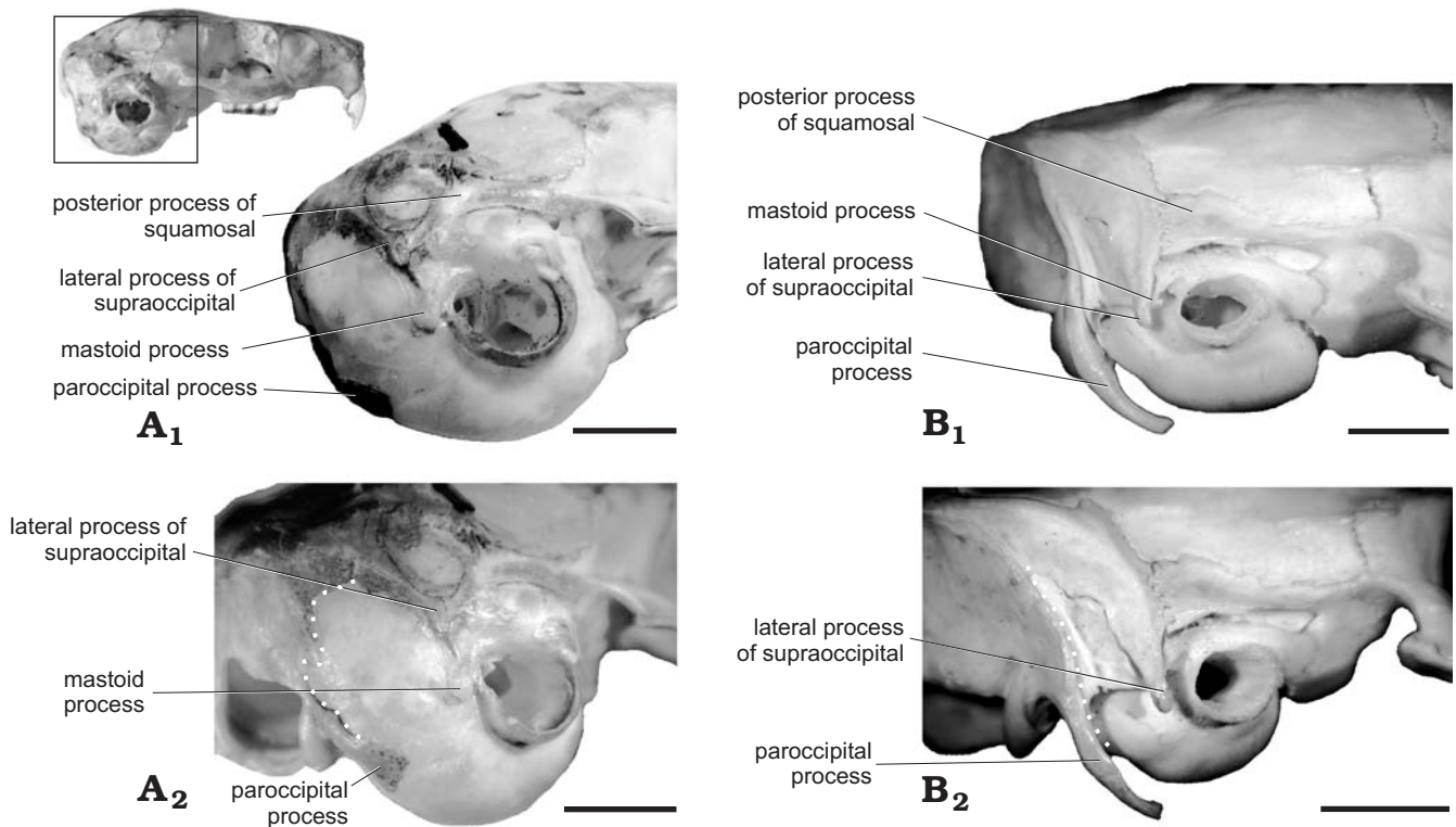
Fig. 3. Lateral (A 1 , B 1 ) and posterolateral (A 2 , B 2 ) views of the temporal region of Recent octodontoids. A. Octomys mimax Thomas, 1920, IMCN-CM 24. B. Proechimys poliopus Osgood, 1914, MLP 22.II.00.7. Dotted line indicates the margin of the supraoccipital. Scale bars 5 mm.
