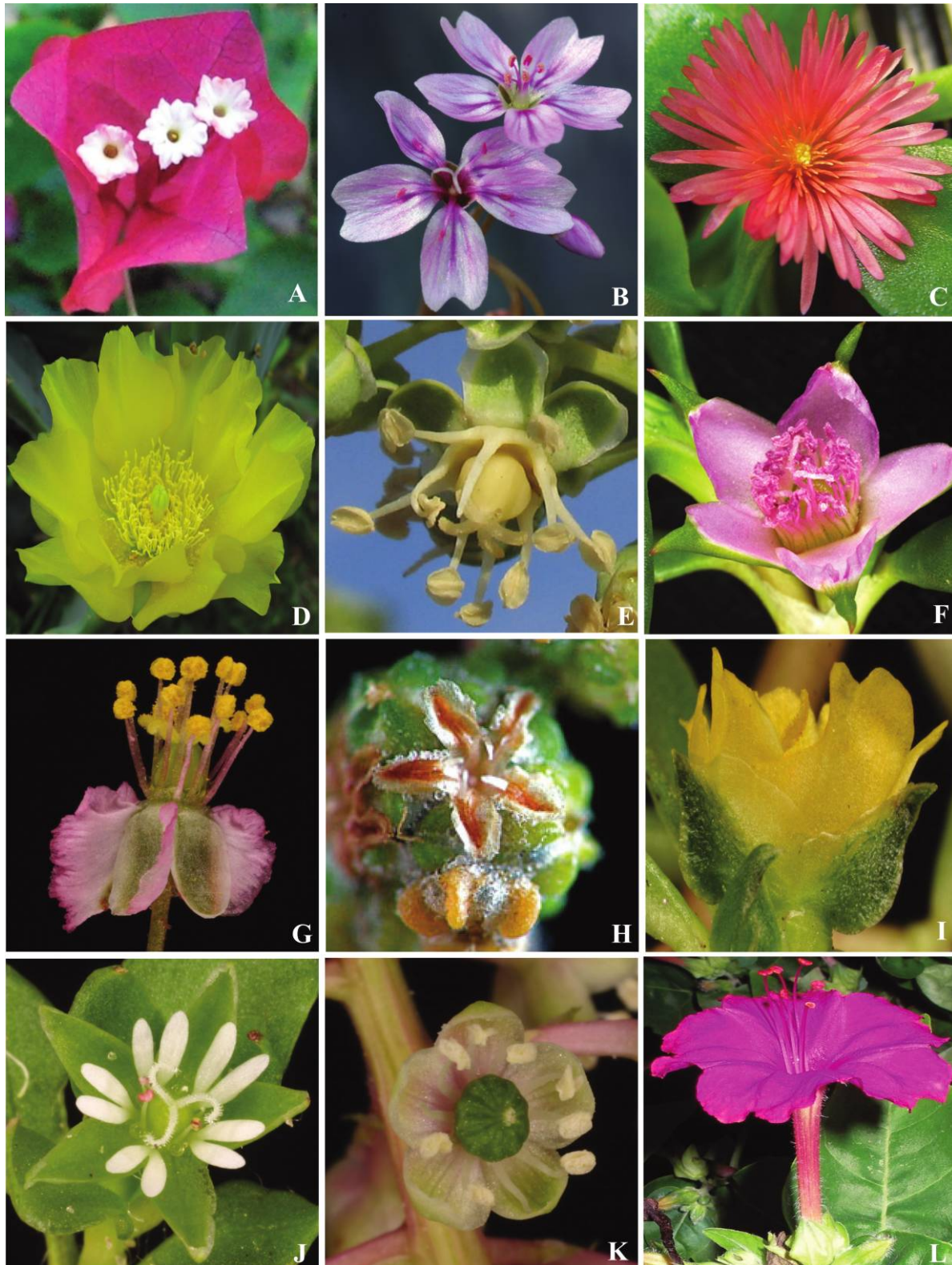
Fig. 4 Diverse forms of perianth in the core Caryophyllales. A, Bougainvillea sp. (Nyctaginaceae); B, Claytonia sp. (photo by Ron Wolf; Portulacaceae s.l.); C, Aptenia cordifolia (Aizoaceae); D, Opuntia humifusa (Cactaceae); E, Stegnosperma sp. (photo by Debra Valov; Stegnospermataceae); F, Sesuvium portulacastrum (Aizoaceae); G, Hypertelis salsoloides (Molluginaceae); H, Chenopodium sp. (photo by Brian Johnston; Amaranthaceae); I, Portulaca oleracea (photo by Kurt Neubig; Portulacaceae); J, Stellaria media (photo by Kurt Neubig; Caryophyllaceae); K, Phytolacca americana (photo by Kurt Neubig; Phytolaccaceae); L, Mirabilis jalapa (photo by Walter Judd; Nyctaginaceae).
