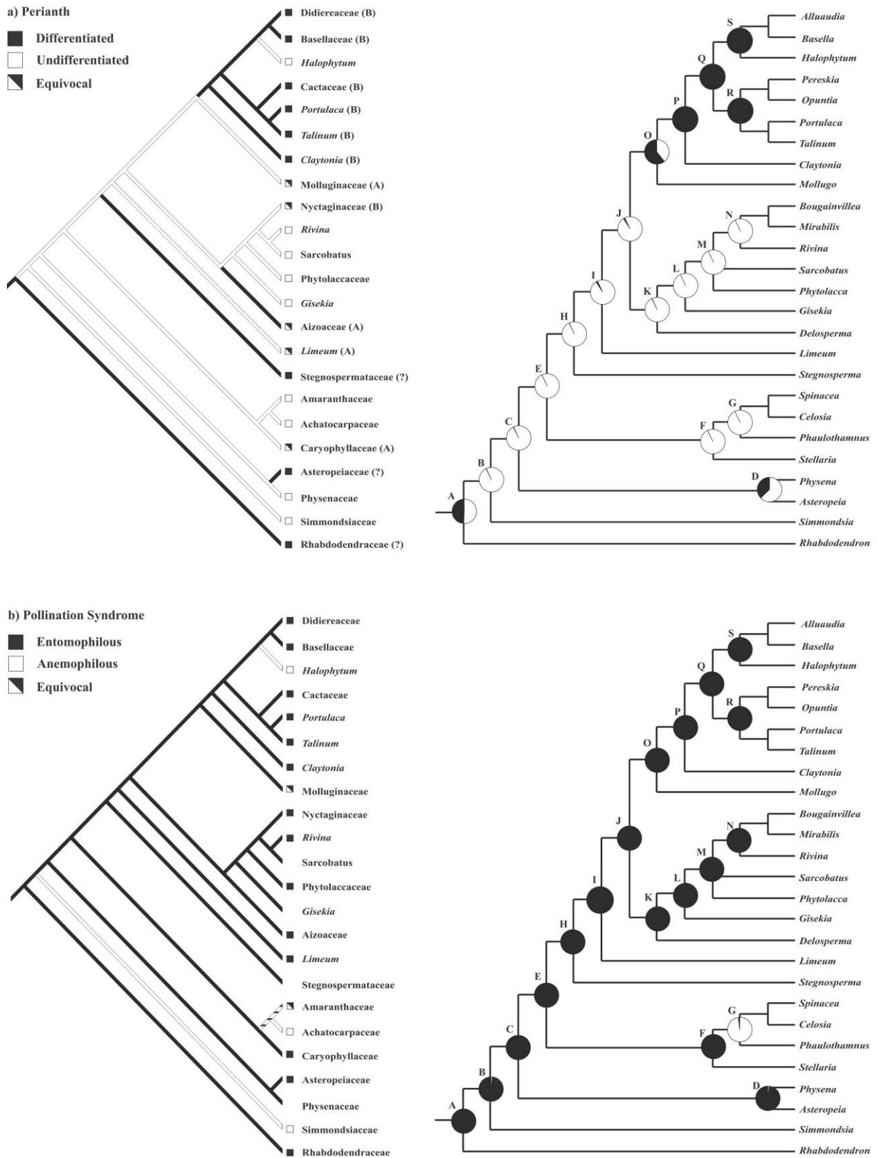
Fig. 3 Parsimony reconstruction (illustrated on a maximum parsimony tree) and stochastic character mapping (illustrated on a Bayesian consensus tree). a. Reconstruction of perianth evolution. b. Pollination syndromes.
