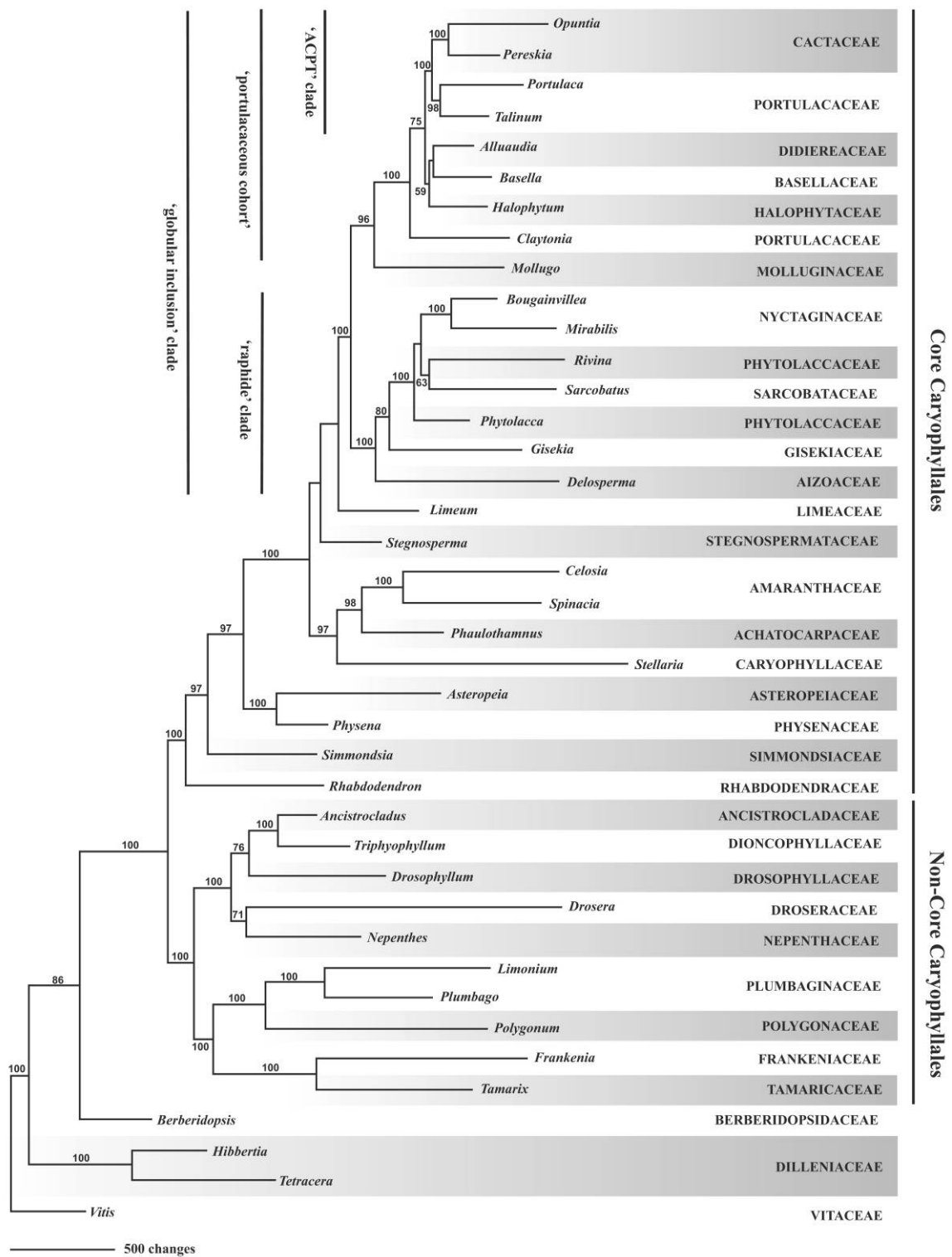
Fig. 2 Phylogram of single most parsimonious tree based on the total evidence data set (two nuclear genes, nine plastid genes from the single-copy region, and the inverted repeat) for 36 members of the Caryophyllales and four outgroups. Numbers above branches are bootstrap values (length 27,604, consistency index 0.605, retention index 0.538).
