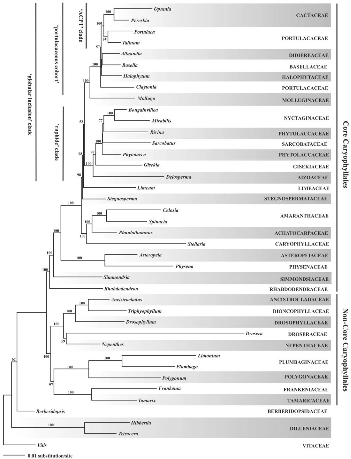
Fig. 1 Maximum likelihood (ML) tree resulting from GARLI analysis of total evidence data set (two nuclear genes, nine plastid genes from the single-copy region, and the inverted repeat) for 36 members of the Caryophyllales and four outgroups. Numbers above branches are bootstrap values ( -\ln L score 210,420.96).
