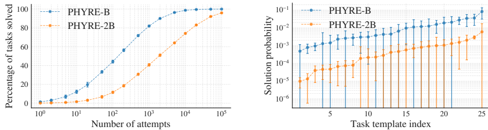
(a) Percentage of tasks solved by a random agent ( y -axis) as a function of the number of attempts ( x -axis; log scale) for both PHYRE tiers.
