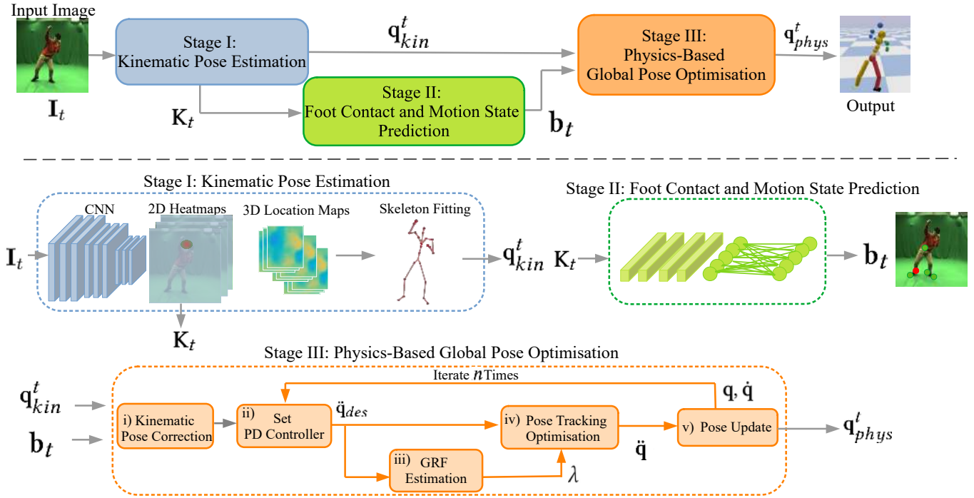
Fig. 3. Overview of our pipeline. In stage I, the 3D pose estimation network accepts RGB image I_t as input and returns 2D joint keypoints K_t along with the global 3D pose q_{kin}^t , i.e. , root translation, orientation and joint angles of a kinematic skeleton. In stage II, K_t is fed to the contact and motion state detection network. Stage II returns the contact states of heels and forefeet as well as a label b_t that represents if the subject in I_t is stationary or not. In stage III, q_{kin}^t and b_t are used to iteratively update the character pose respecting physics laws. After the n pose update iterations, we obtain the final 3D pose q_{phys}^t . Note that the orange arrows in stage III represent the steps that are repeated in the loop in every iteration. Kinematic pose correction is performed only once at the beginning of stage III.
