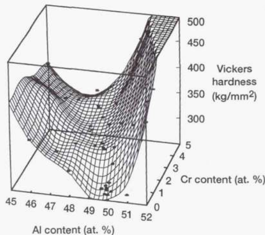
Figure 6.—Combined effect of stoichiometry and Cr additions on the hardness of Cr-doped B2 NiAl alloys (Cotton, Noebe, and Kaufman 1993a).
