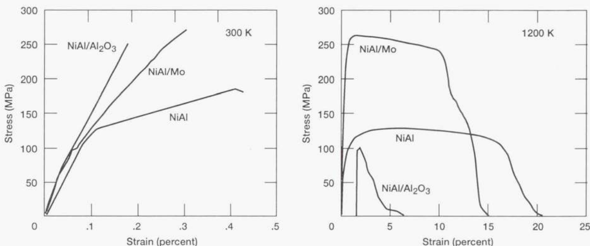
Figure 24.—Tensile stress-strain curves for NiAl, NiAl/ \text{Al}_2\text{O}_3 , and NiAl/Mo composites at 300 and 1200 K (Bowman 1992a).
