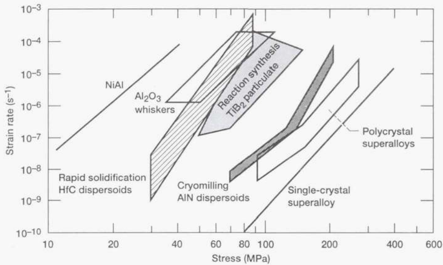
Figure 18.—Effect of composite strengthening and second-phase reinforcement on the creep behavior of NiAl at 1300 K.
