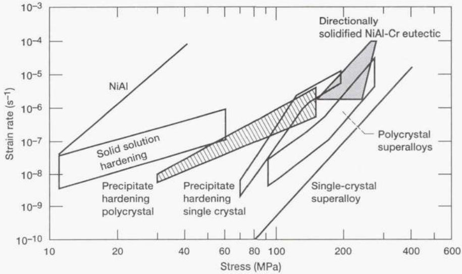
Figure 17.—Effects of alloying on the creep behavior of NiAl at 1300 K. Both solid-solution alloys and precipitation-hardened NiAl-based materials are included in the figure.
