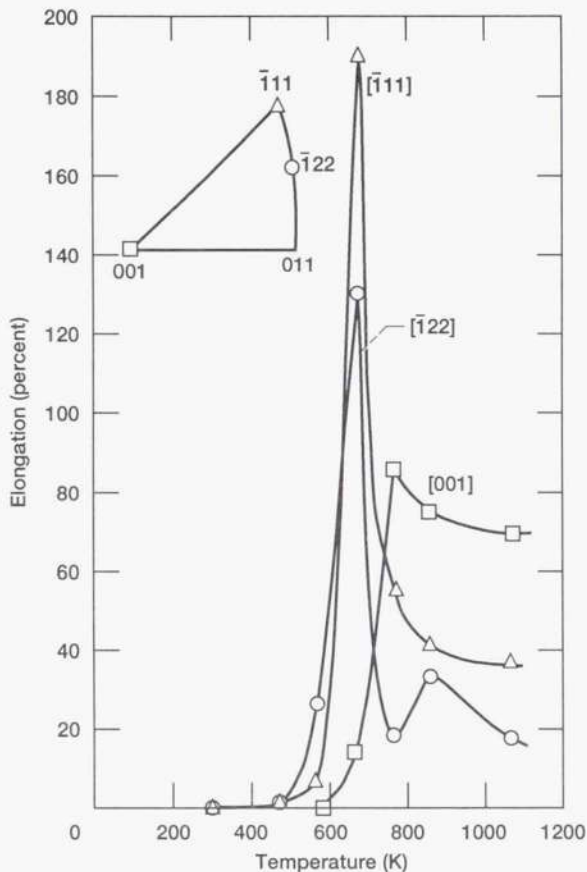
Figure 9.—Effect of temperature on the tensile ductility of NiAl single crystals (Takasugi, Wantanabe, and Hanada 1992).
