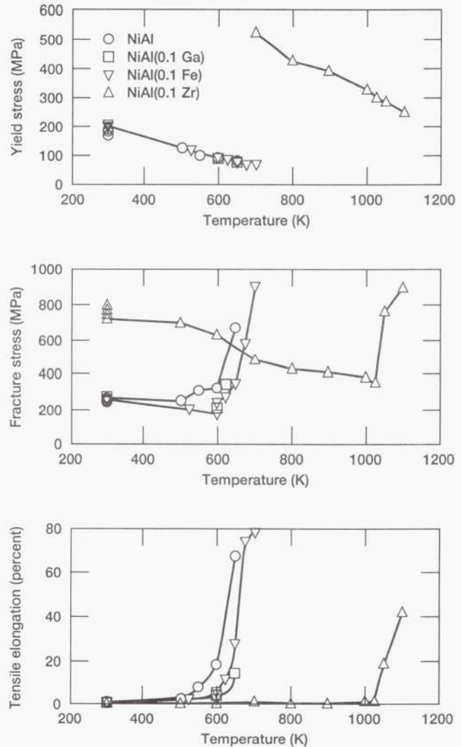
Figure 14.—Effect of test temperature on the 0.2-percent offset yield stress, fracture stress, and tensile elongation of NiAl microalloyed with 0.1 at.% Ga, Fe, or Zr (Noebe and Behbehani 1992).
