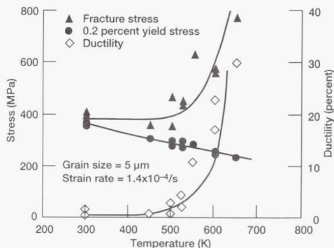
Figure 11.—Effect of test temperature on the yield stress, fracture stress, and tensile elongation of power-extruded NiAl (Noebe et al. 1991).
