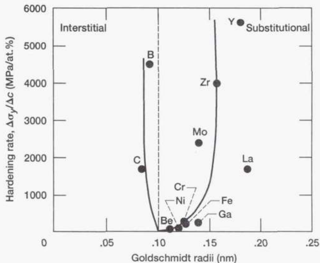
Figure 5.—Relation between hardening rate and element size for various alloying additions in NiAl.
