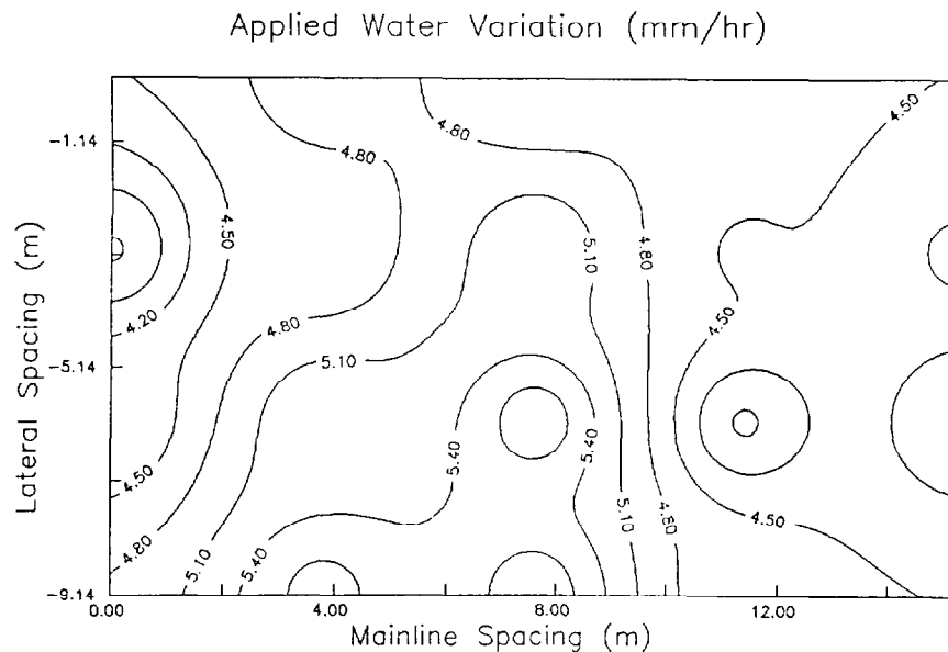
Fig. 2. Spatial variability of the applied water (millimeters per hour) between four sprinkler heads (uniformity coefficient is 0.88), as computed by the network of catch cans.
