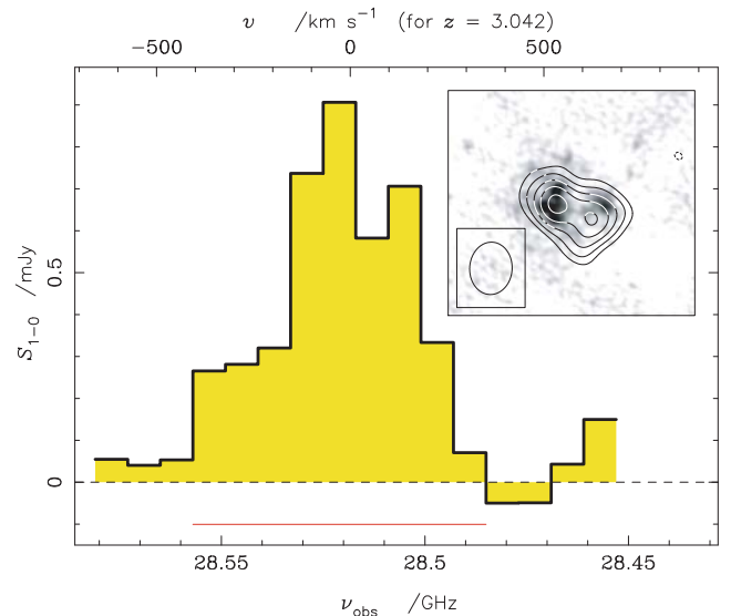
Figure 1. Spectrum of ^{12}\text{CO} J = 1-0 line emission from SDP.81 from the Expanded Very Large Array. Inset: Contours of the CO(1–0) emission, integrated across the velocity range -400 to +350 \text{km s}^{-1} (indicated by the line below the spectrum, and where v = 0 \text{km s}^{-1} at 28.51836 GHz for z = 3.042 ), which corresponds roughly to the FWZI of the line, overlaid upon a grey-scale SMA 880 \mu\text{m} continuum image (scaled from 0–8 mJy) presented by Negrello et al. (2010). The synthesized beam for the CO observations is shown in the inset, bottom left ( 3.3 \times 2.4 arcsec 2 ), and the contours are plotted at -2.5, 2.5, 3.5, \dots, 6.5 \times \sigma , where the rms noise level, \sigma = 100 \mu\text{Jy beam}^{-1} . The synthesized beam for the continuum observations is \approx 12 \times 8 arcsec 2 and the size of the image is 20 \times 20 arcsec 2 .
