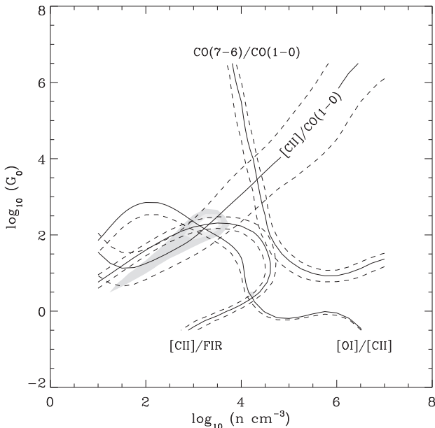
Figure 5. PDR model predictions for the density ( n ) and the FUV flux ( G_0 ) from the observed line ratios. The [\text{O I}] 63 \mu\text{m}/[\text{C II}] 158 \mu\text{m} is shown as an upper limit, the dashed line indicating the side where we expect the ratio to be if [\text{O I}] is less luminous. The shaded contours show the 3\sigma confidence region of the expected (n, G_0) values when considering only [\text{C II}] , \text{CO}(1-0) and the upper limit on [\text{O I}] . The \text{CO}(7-6)/\text{CO}(1-0) ratio was corrected for [\text{C I}] blending with \text{CO}(7-6) .
