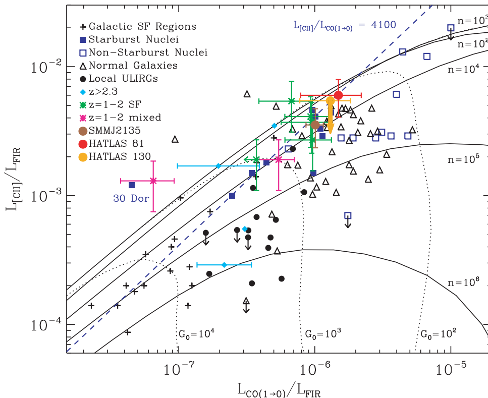
Figure 4. Diagnostic diagram of L_{[C\text{II}]} / L_{\text{FIR}} as a function of L_{\text{CO}(1-0)} / L_{\text{FIR}} for SDP.81 (the rightmost filled circle) and SDP.130 (filled circle with a down arrow), compared to local and other known high-redshift galaxies of different classes (Stacey et al. 1991, 2010; Hailey-Dunsheath et al. 2010). The lines with the constant density n and constant G_0 from PDR models of Kaufman et al. (1999) are also shown. The [C II] luminosity was corrected for the fraction of the flux arising from H II and diffuse ionized regions. The CO(1–0) line flux from the EVLA measurement was multiplied by 2 to take into account that the line is optically thick and we see only the fraction coming from the illuminated PDR side. L_{[C\text{II}]} / L_{\text{CO}(1-0)} of 4100, typical for local starburst galaxies, is also shown as a dashed line. We have used L_{\text{FIR}}(42.5\text{--}122.5 \mu\text{m}) = L_{\text{IR}}(3\text{--}2000 \mu\text{m}) / 1.54 , derived by integrating the SED of SDP.81.
