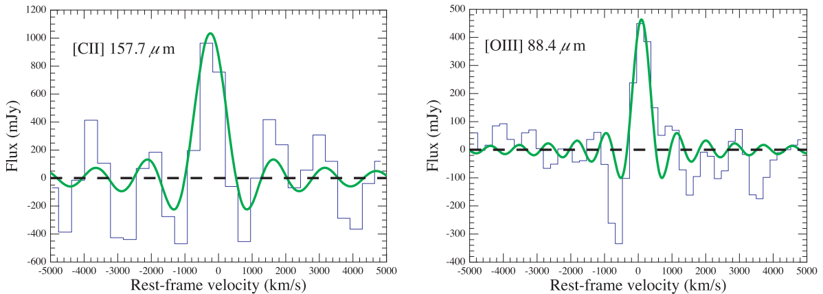
Figure 3. Continuum-subtracted regions within \pm 5000 \text{km s}^{-1} rest frame for [C II] 157.7 \mu\text{m} (left-hand panel) and [O III] 88.4 \mu\text{m} (right-hand panel) lines of SDP.81. The FTS data processed using two reference dark-sky observations (see Section 3) are shown as a histogram. The dashed line indicates the zero level. The best-fitting sinc function is also shown.
