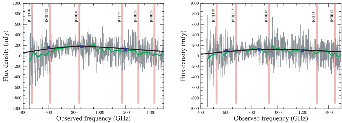
Figure 2. The FTS high- and low-resolution spectra of SDP.81 (left-hand panel) and SDP.130 (right-hand panel) overlaid with the three SPIRE photometric points (dots) and the SED template fit. The photometric errors, even including the 7 per cent flux calibration uncertainty of the SPIRE Photometer, are smaller than the dots. The expected positions of a number of fine-structure lines are indicated with vertical bars.
