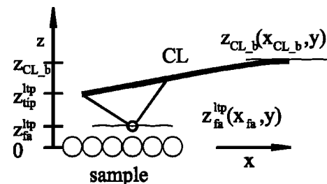
FIG. 1. Schematic of an oscillating cantilever (CL) with tip and front atom (fa) at its lower turnaround point (ltip) close to a sample.
