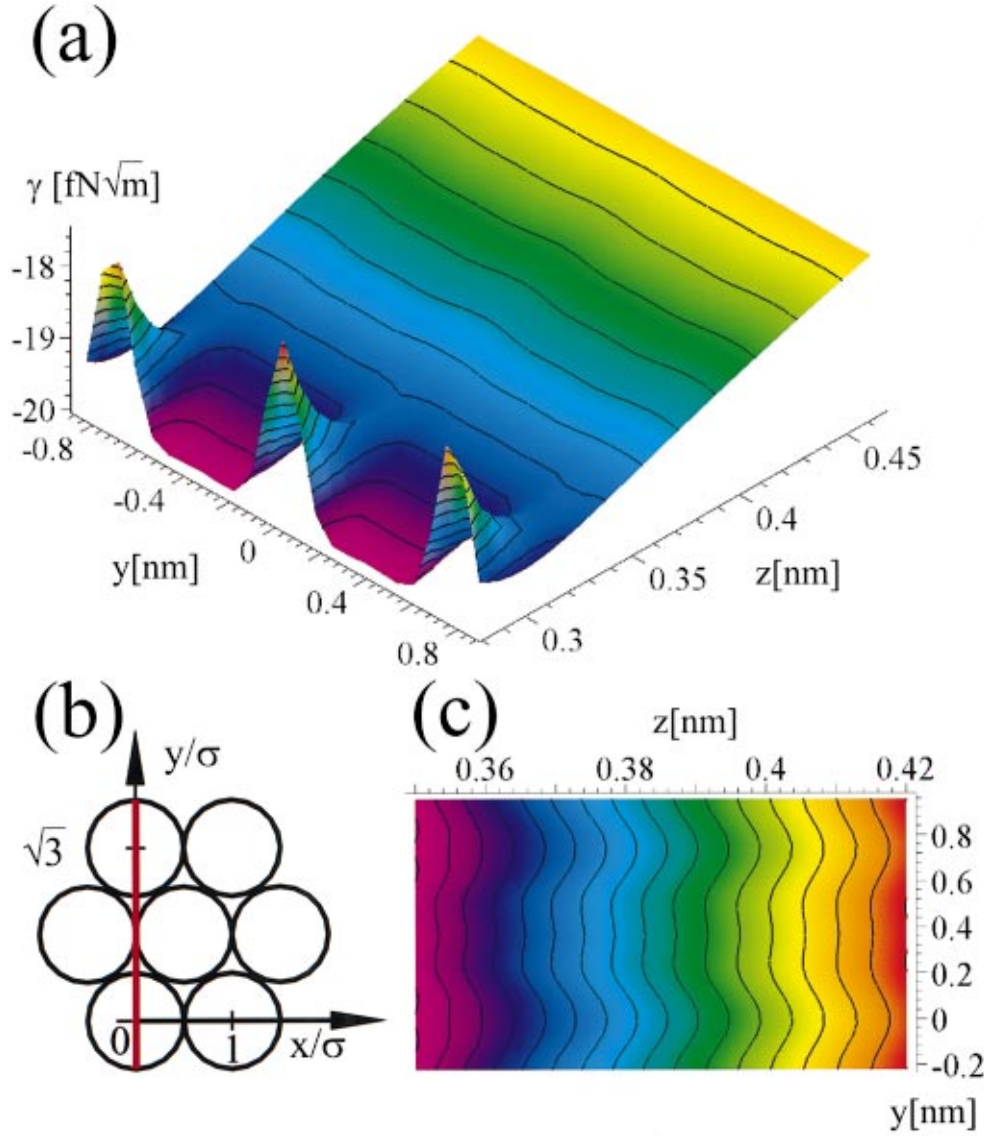
FIG. 3. (Color) (a) Normalized frequency shift \gamma_{IA}(x=0,y,z) from y=-2\sigma to 2\sigma ( \sigma=0.43 nm). Xenon atoms are situated at y=0,\pm\sqrt{3}\sigma . The contour lines of constant \gamma are cross sections of the corresponding FM-AFM image z(x,y,\gamma) . Maximal corrugation is obtained for \gamma \approx -18 fN \sqrt{\text{m}} (green area). (b) Arrangement of Xenon atoms on the surface, (c) top view of \gamma_{IA} along red track in (b) showing a maximal corrugation of \sim 5 pm.
