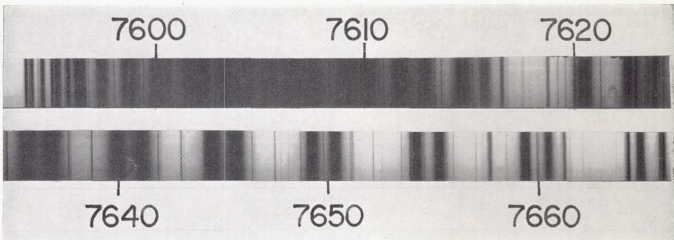
Spectrum of 0.76-Micron Oxygen Band , obtained with the 150-ft tower telescope at Mt. Wilson. In the upper part is the band head (left); the R branch lies between the band head and the band center; three lines of the P branch can be seen to the right of the band center. In the lower part are lines farther out in the P branch. The very narrow lines throughout are from the isotopic molecules O^{17} and O^{18} . There are also some solar lines.
