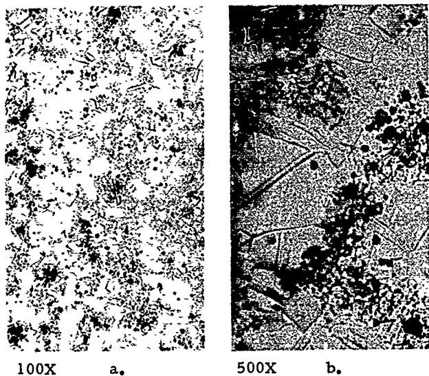
FIGURE 25. TRANSVERSE CROSS SECTION OF ALLOY 718 BAR ANNEALED AT 1800 F AND DOUBLE AGED
