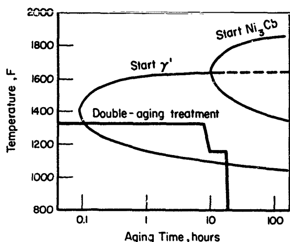
FIGURE 42. ISOTHERMAL-TRANSFORMATION DIAGRAM FOR GAMMA PRIME ( \gamma' ) AND Ni_3Cb PHASES IN ALLOY 718; WITH DOUBLE-AGING TREATMENT SUPERIMPOSED (After Eiselstein) (6)
