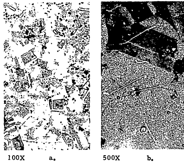
FIGURE 26. TRANSVERSE CROSS SECTION OF ALLOY 718 BAR ANNEALED AT 1950 AND DOUBLE AGED
