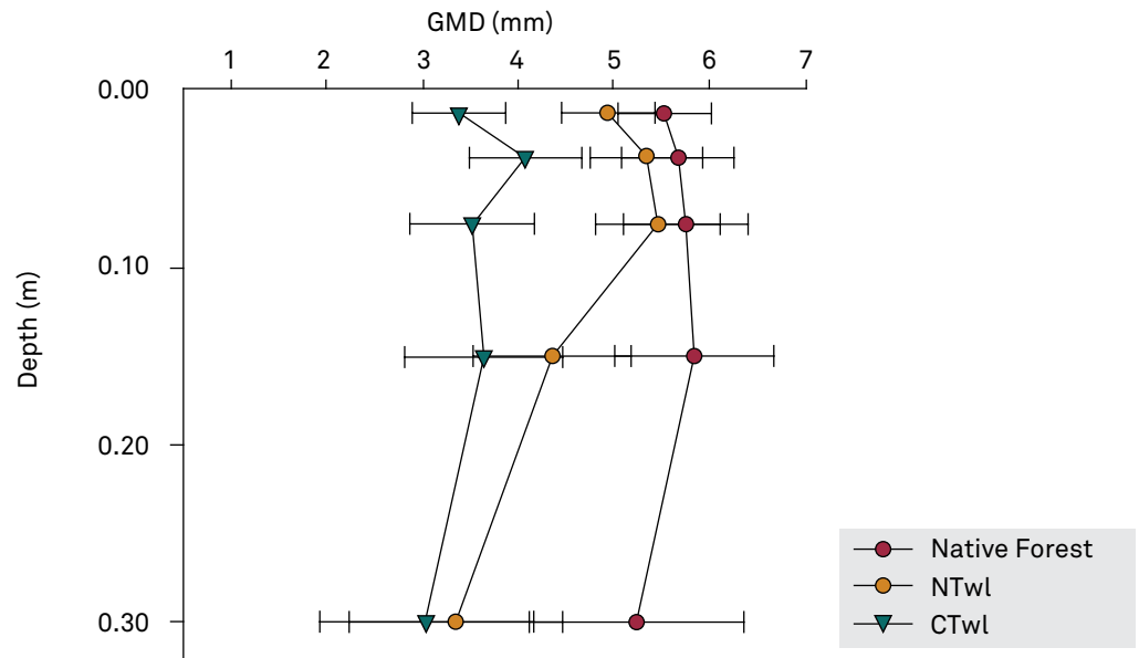
Figure 3. Geometric mean diameter (GMD) of the soil aggregates as affected by soil use and tillage systems in a Latosolo Bruno Alumínico típico (Hapludox). Horizontal bars indicate the interval of least significant difference for the t test and their overlap in the same soil layer means the absence of differences between the averages of the systems. CTwl: conventional tillage without lime; and NTwl: no-tillage without lime.
