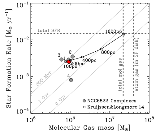
Figure 10. Molecular gas depletion time, \tau_{\text{dep}} , the ratio of molecular gas mass to star formation rate, as a function of spatial scale: ranging from individual star-forming complexes ( d \approx 100 pc) to the entire star-forming disk of NGC 6822 ( d \approx 1600 pc). The Kruijssen & Longmore (2014) model provides an estimate of the bias in t_{\text{dep}} when selectively focusing on star-forming regions (black curve). We infer that globally, NGC 6822 may have t_{\text{dep}} \approx 2 Gyr (similar to massive disk galaxies) and molecular gas mass M_{\text{mol}} \approx 2 \times 10^7 M_{\odot} .
