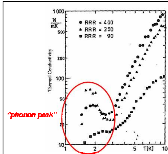
Figure 3: Thermal conductivity of various RRR samples
