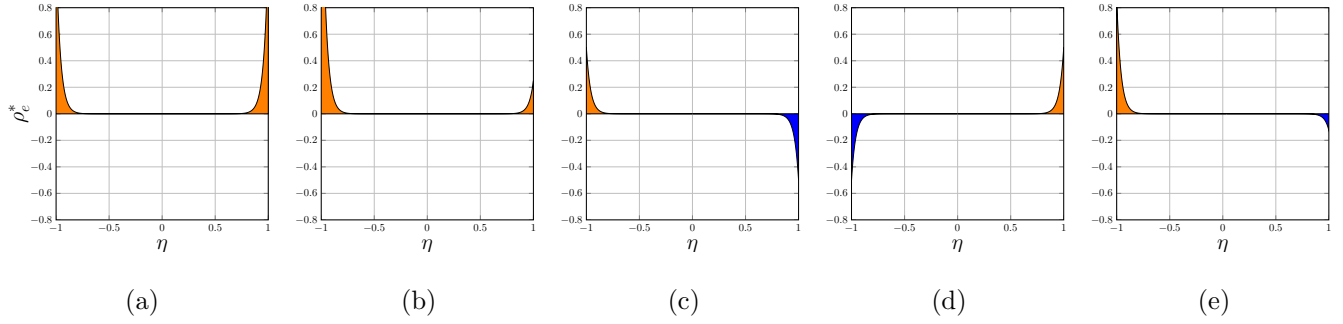
FIG. 1. Charge density distribution \rho_e^* (normalized) along the domain cross-section, in an electrolytic solution enclosed by walls; potential difference between right and left walls is \delta ; the net charge in the cross-section is q_0 (normalized). For each case, inverse of scaled Debye length \kappa = 25 . (a): q_0 = 0.1 and \delta = 0 . (b): q_0 = 0.1 and \delta = 2 . (c): q_0 = 0 and \delta = 1 (d): q_0 = 0 and \delta = -1 (e): q_0 = 0.03 and \delta = 2
