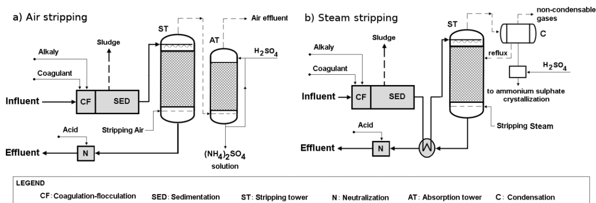
Figure 2. Typical flow diagrams of the stripping processes with air (a) and steam (b).
