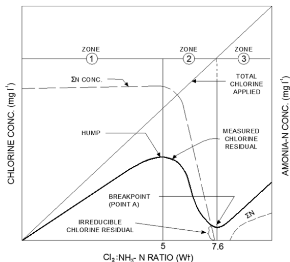
Figure 8. Theoretical breakpoint curve.
