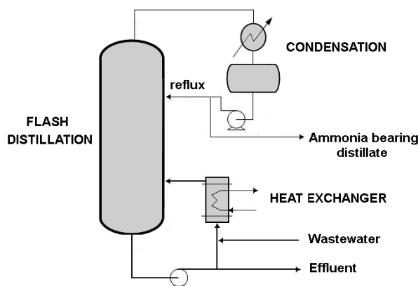
Figure 4. Diagram of a typical flash distillation process for ammonia recovery.
