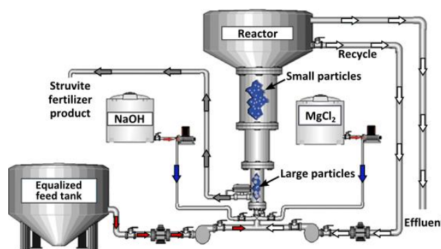
Figure 6. Diagram of the process for struvite precipitation and recovery.
