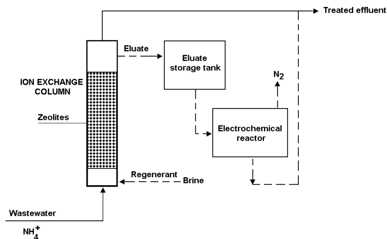
Figure 7. Simplified diagram of a ion exchange process on a zeolite bed for ammonia removal. Ammonia in the eluate is decomposed to nitrogen gas by an electrochemical reaction.
