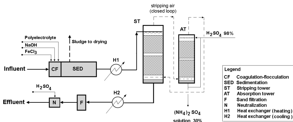
Figure 3. Diagram of a physico-chemical process for leachate treatment, with wastewater pre-heating and a closed-loop air stripping process.
