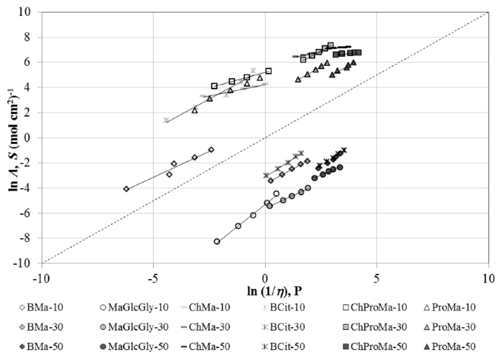
Fig. 6 – Walden plot for NADES
