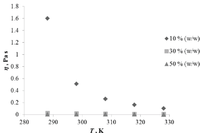
Fig. 4 – Viscosity of ChMa with different water content as function of temperature
