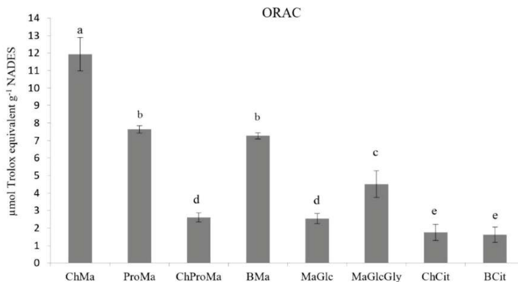
Fig. 9 – Oxygen radical absorbance capacity (ORAC) of prepared NADES. Results (mean values, n = 3 , \pm SD) are expressed as \mu\text{mol TE g}^{-1}
