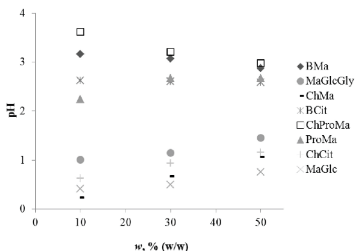
Fig. 5 – pH values of NADES as function of water content at 298 K
