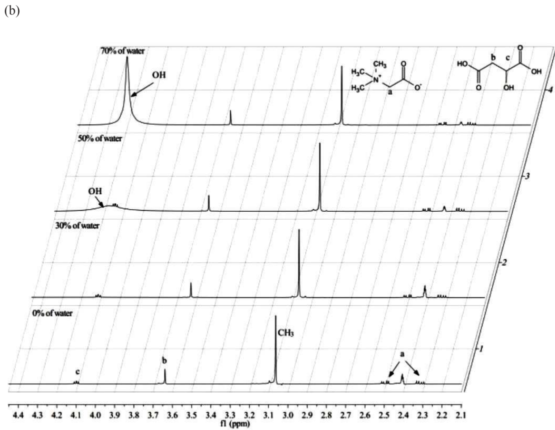
Fig. 2 – NMR spectra of ChMa (a) and BMa (b) prepared with different amounts of water (0 to 70 % by weight)
