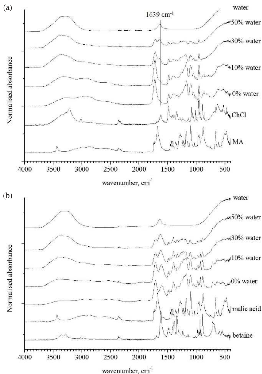
Fig. 1 – FTIR spectra of ChMa (a) and BMa (b) prepared with different amounts of water (0 to 50 % by weight)
