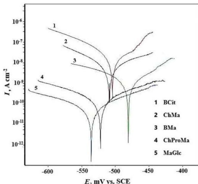
Fig. 7 – Potentiodynamic polarization curves obtained for steel X6CrNiTi18-10 in NADES with 50 % (w/w) water at 25 °C
