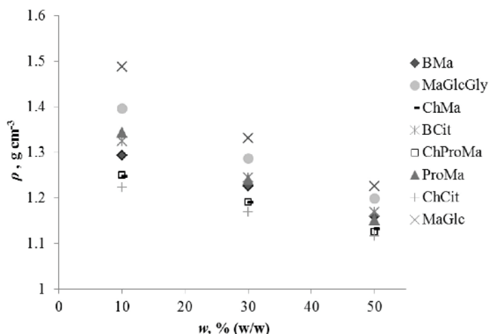
Fig. 3 – Densities of NADES as function of water content at 298 K
