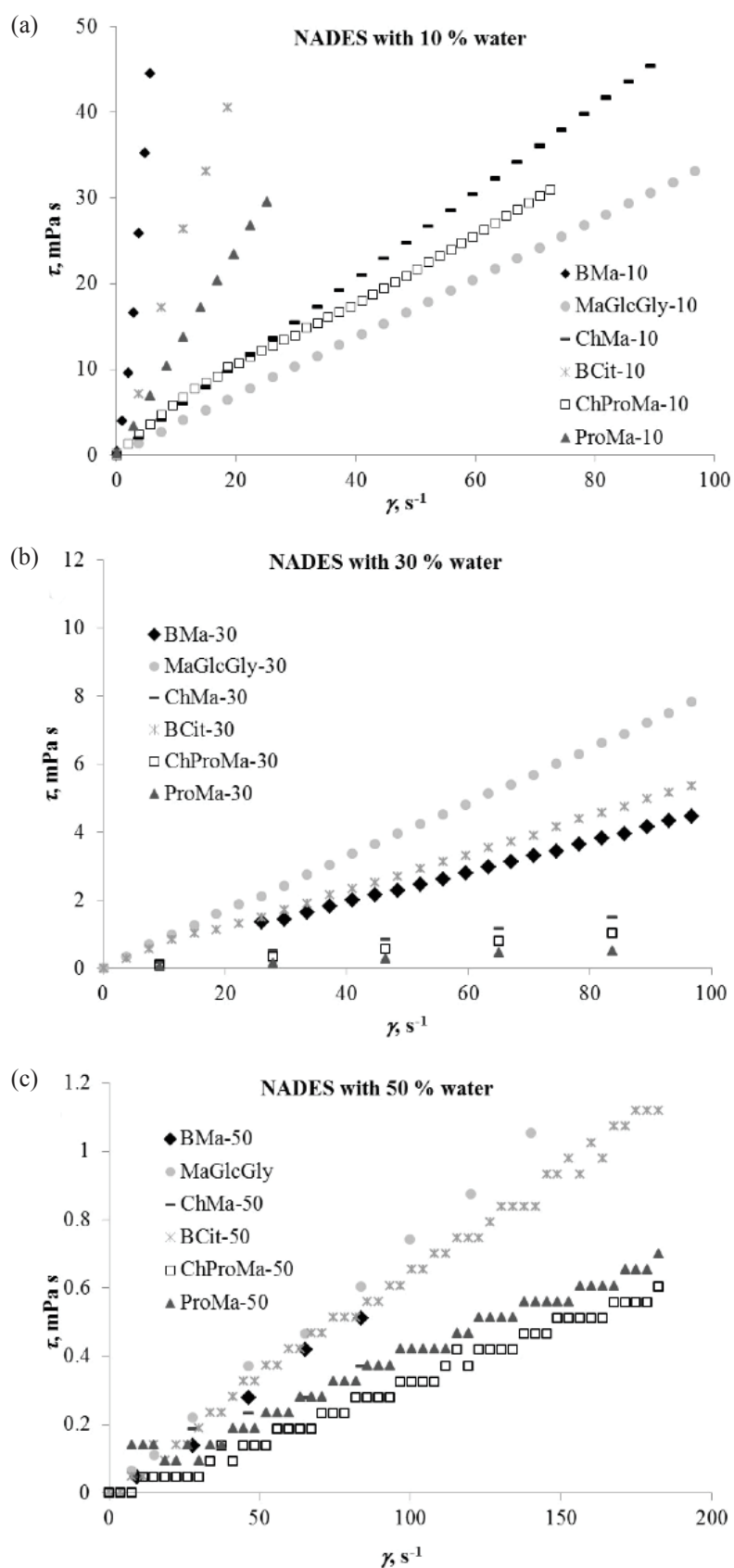
Fig. 1S – Influence of shear stress, \tau on shear rate, \gamma for NADES with 10 % (w/w) (a), 30 % (w/w) (b), 50 % (w/w) (c) water
