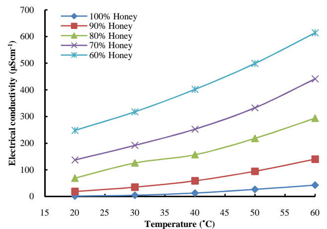
Fig. 2: Variations of electrical conductivity at different temperatures
