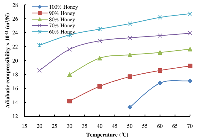
Fig. 6: Variations of adiabatic compressibility at different temperatures
