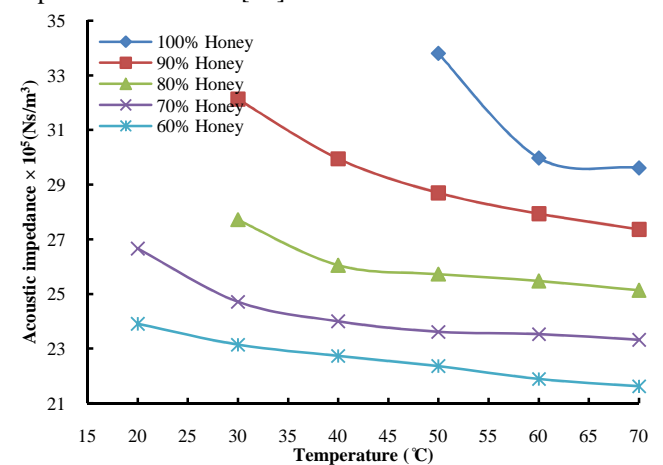
Fig. 7: Variations of acoustic impedance at different temperatures
