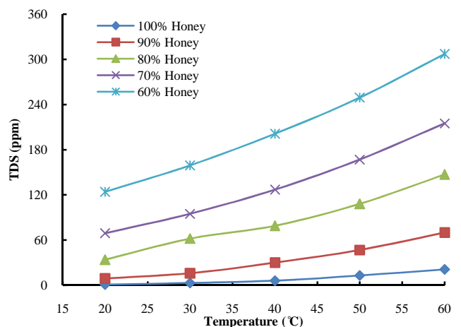
Fig.3: Variations of TDS at different temperatures
