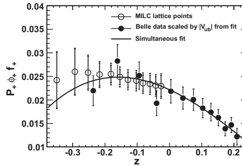
Fig. 20. |V_{ub}| extraction from a simultaneous fit to experimental (closed circles) and FNAL/MILC lattice QCD results (open circles).
