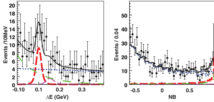
Fig. 16. Signal for B^\pm \rightarrow DK^\pm decays from Belle ADS analysis. In these \Delta E and NB (continuum suppression variable) distributions, [K^+\pi^-]_D K^- components are shown by thicker dashed curves (red).
