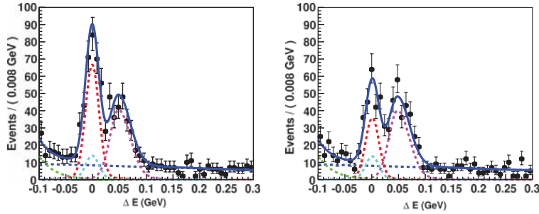
Fig. 15. Signals for B^\pm \rightarrow D_1 K^\pm decays. The left (right) figure is for B^- ( B^+ ) decays. The plotted variable, \Delta E , peaks at zero for signal decays, while background from B^\pm \rightarrow D\pi^\pm appears as a satellite peak at positive values.
