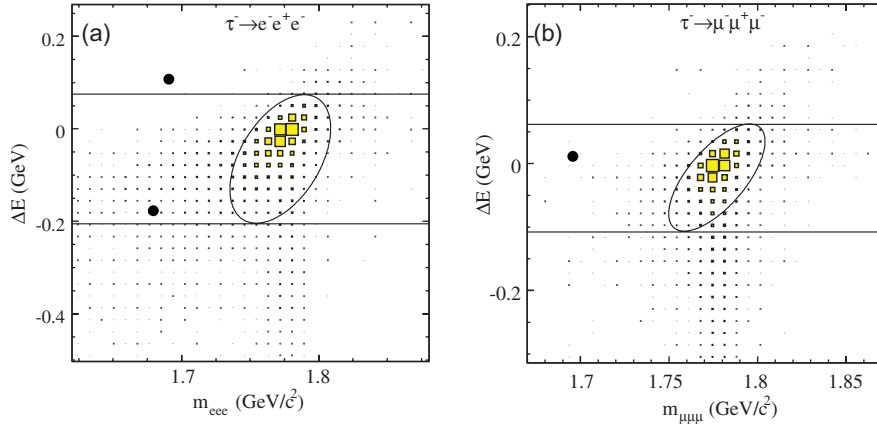
Fig. 33. M_{\ell\ell\ell}-\Delta E distributions for (a) \tau^- \rightarrow e^- e^+ e^- and (b) \tau^- \rightarrow \mu^- \mu^+ \mu^- modes [224]. The black dots and shaded boxes show the data and signal MC, respectively. The ellipse is the signal region. The region formed by the two parallel lines, excluding the signal ellipse region, is the side-band region used to evaluate the expected number of backgrounds in the signal region.
