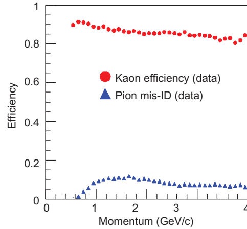
Fig. 2. Kaon identification efficiency and fake rate as a function of momentum.
