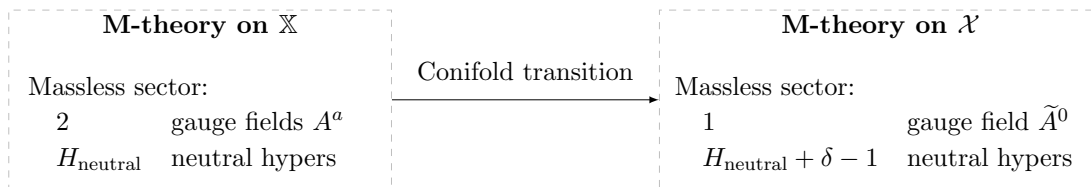
Figure 5. The two theories obtained by compactifying M-theory on \mathbb{X} and \mathcal{X} , respectively, are connected by a conifold transition.
