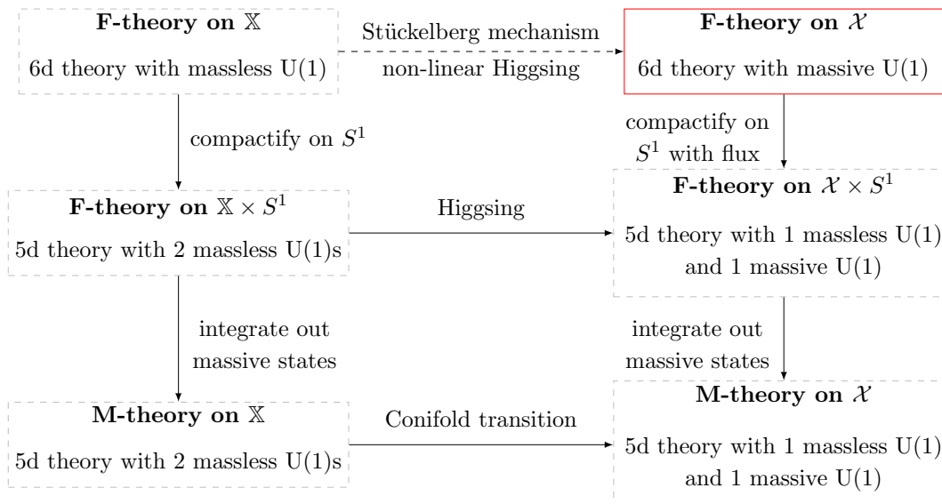
Figure 1. Overview of our discussion. The object of interest in the top-right corner, corresponding to the six-dimensional theories coming from F-theory on a space without section \mathcal{X} . In the examples we will discuss explicitly these compactifications are closely related (by making some fields massive) to F-theory on spaces with section \mathbb{X} , giving the six-dimensional theories in the top-left corner. Compactification of these theories on S^1 gives two five-dimensional theories, in the middle row, which can also be obtained by M-theory on the corresponding Calabi-Yau threefolds (shown in the bottom row). The five-dimensional theories are related by Higgsing, or equivalently, by conifold transitions in M-theory.
