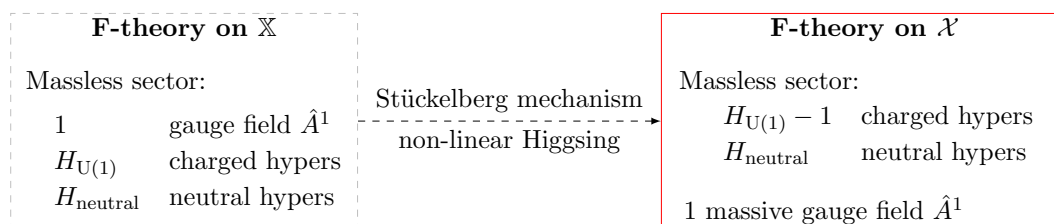
Figure 2. Six-dimensional effective theories with a massless and massive U(1) gauge field.
