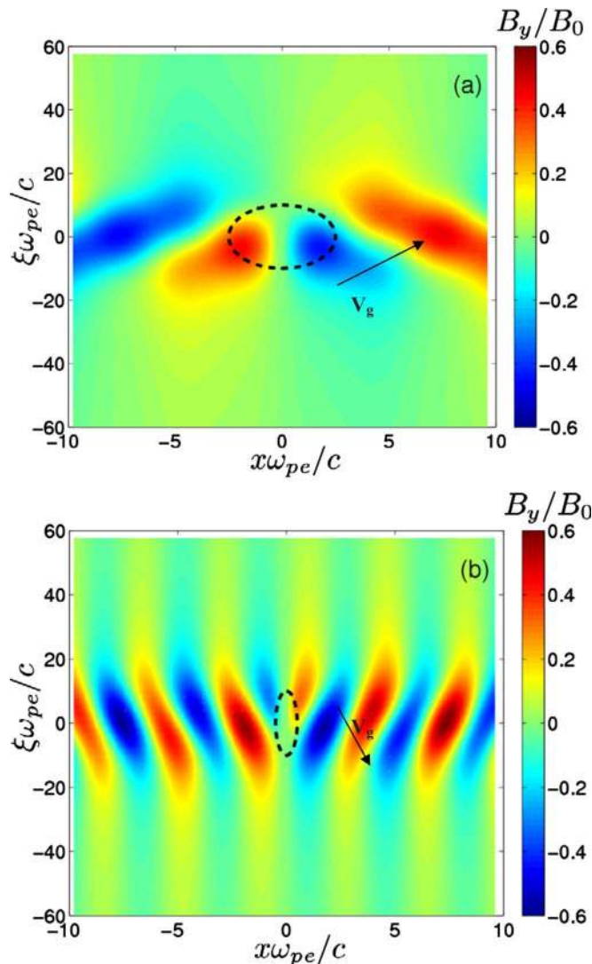
FIG. 13. (Color online) Plots of the steady-state amplitude of the transverse magnetic field perturbations B_y . The beam-plasma parameters correspond to Z_b=1 , l_b=10c/\omega_{pe} , \beta_b=0.33 , and n_p=2.4 \times 10^{11} \text{ cm}^{-3} . The applied magnetic field, B_z=1600 \text{ G} , corresponds to \omega_{ce}/(2\beta_b\omega_{pe})=1.54 . The frames in the figure show (a) excitation of primarily long-wavelength electromagnetic waves by a wide-aperture ion beam with r_b=2.5c/\omega_{pe} and (b) excitation of primarily short-wavelength quasiolestatic waves by a thin beam with r_b=0.5c/\omega_{pe} . The normalization factor in (a) and (b) is given by B_0=4\pi n_{b0}Z_b e\beta_b r_b . The arrows schematically illustrate the direction of the wave packet group velocity. The dashed lines correspond to the contours of constant beam density corresponding to the effective beam radius r_b .
