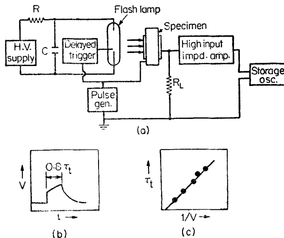
Figure 2. (a) Experiment for drift mobility measurement in ionic materials. (b) Output voltage vs. time, giving transit time. (c) Transit time \tau_t vs. 1/V where V = applied drift voltage.
