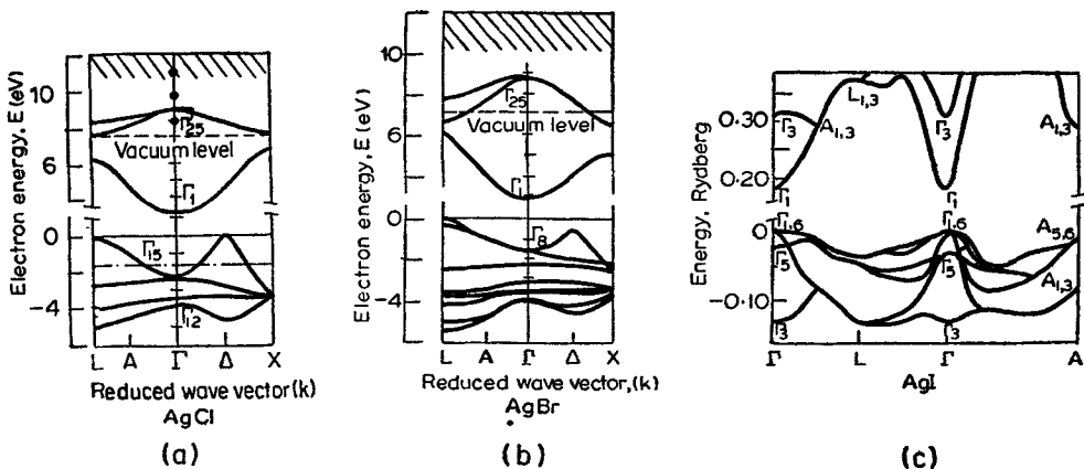
Figure 4. (a) Band-structure of AgCl. (b) Band-structure of AgBr. (c) Band-structure of AgI.
