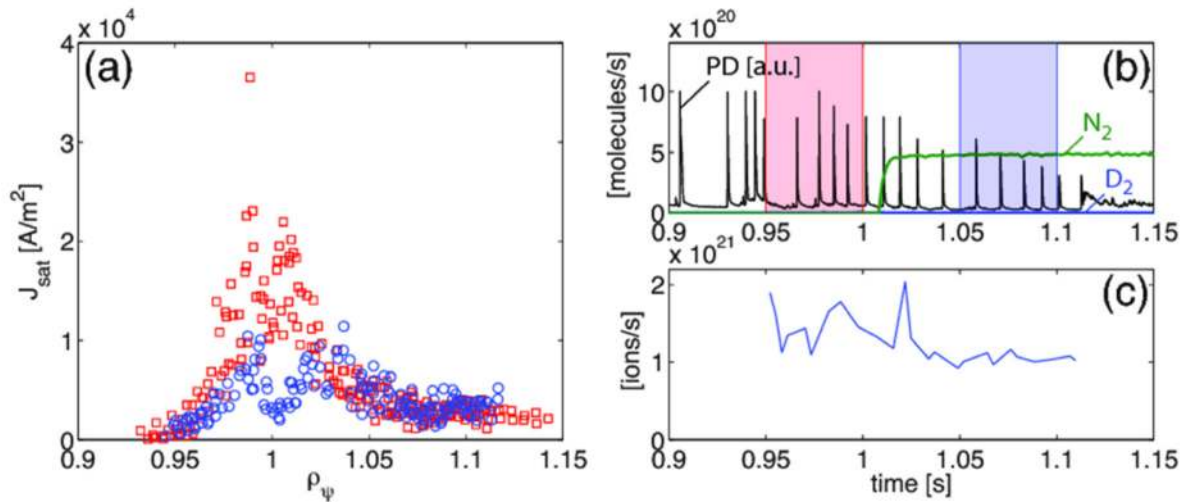
Figure 8. Effect of nitrogen seeding on inter-ELM outer-target saturation-current profiles: (a) ion-saturation profiles from LPs in intervals before and after seeding; (b) D_\alpha photodiode signal and nitrogen and deuterium injection rates; (c) integrated ion flux to outer target. Reproduced with permission from [77].
