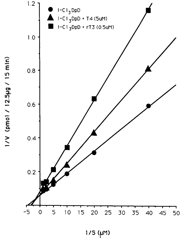
Figure 1. Kinetics of [ ^{125} I]Cl _3 DpD deiodination by liver microsomes and inhibition by rT _3 and T _4 . Double reciprocal plot of rate of deiodination versus [ ^{125} I]Cl _3 DpD concentration in the absence ( \bullet ) or presence of T _4 ( \blacktriangle ) or rT _3 ( \blacksquare ). Deiodinase activity was determined as described in Methods.
