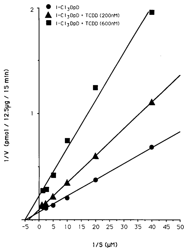
Figure 2. Kinetics of [ 125 I]Cl 3 DpD deiodination by liver microsomes and inhibition by TCDD. Double reciprocal plot of rate of deiodination versus [ 125 I]Cl 3 DpD concentration in the absence (●) or presence of 200 nM (▲) or 600 nM TCDD (■). Deiodinase activity was determined as described in Methods.
