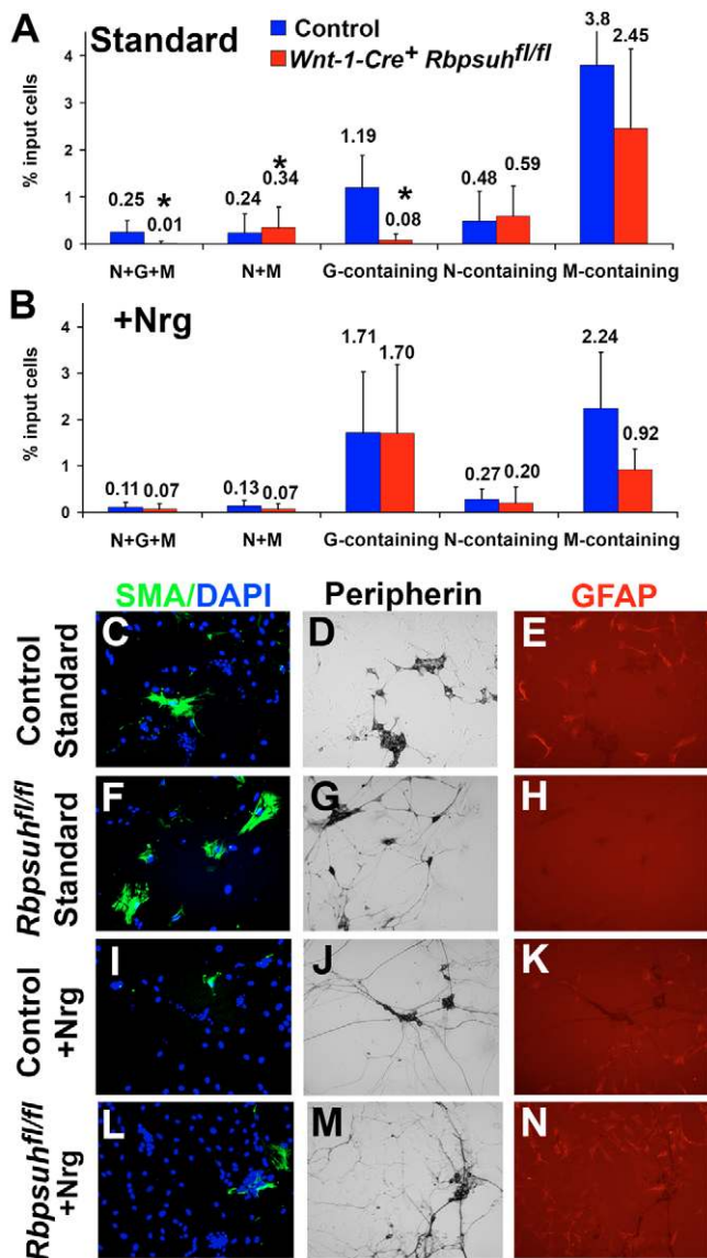
Fig. 3. Neural crest progenitors with glial potential persist in Wnt1-Cre + Rbpsuh fl/fl sensory ganglia despite the lack of gliogenesis in vivo, but require stimulation by a gliogenic factor to undergo gliogenesis in culture. (A-N) We dissociated and cultured dorsal root ganglion cells from E13.5 control and Wnt1-Cre + Rbpsuh fl/fl mouse embryos at clonal density (500 cells per 35 mm dish) under adherent conditions. (A,B) Multilineage colonies (N+G+M) contained neurons (N, peripherin + ), glia (G, Gfap + ) and myofibroblasts [M, Sma + (Acta2/Actg1 – Mouse Genome Informatics)]. Other colonies were also counted. The data are expressed as the percentage of cells added to culture that formed each type of colony. Wnt1-Cre + Rbpsuh fl/fl cells formed significantly fewer multilineage and glia-containing (G-containing) colonies (which included all multilineage, glia-only, and other colonies that contained glia) as compared with control cells (A; *, P < 0.05 ). Wnt1-Cre + Rbpsuh fl/fl cells did not differ from control cells in their ability to form neuron-containing or myofibroblast-containing colonies (A). Addition of the gliogenic factor neuregulin (Nrg) to sister cultures allowed Wnt1-Cre + Rbpsuh fl/fl cells to form normal numbers of multilineage, glia-containing and other types of colonies as compared with control cells (B). (C-N) Representative photos of single fields of view from within multilineage colonies cultured from control cells in standard medium (C-E), Wnt1-Cre + Rbpsuh fl/fl cells in standard medium (F-H), control cells in the presence of Nrg (I-K) and Wnt1-Cre + Rbpsuh fl/fl cells in Nrg (L-N) show that Rbpsuh -deficient NCSCs rarely formed glia (H, Gfap, red), except in the presence of Nrg (N) (three to six independent experiments).
