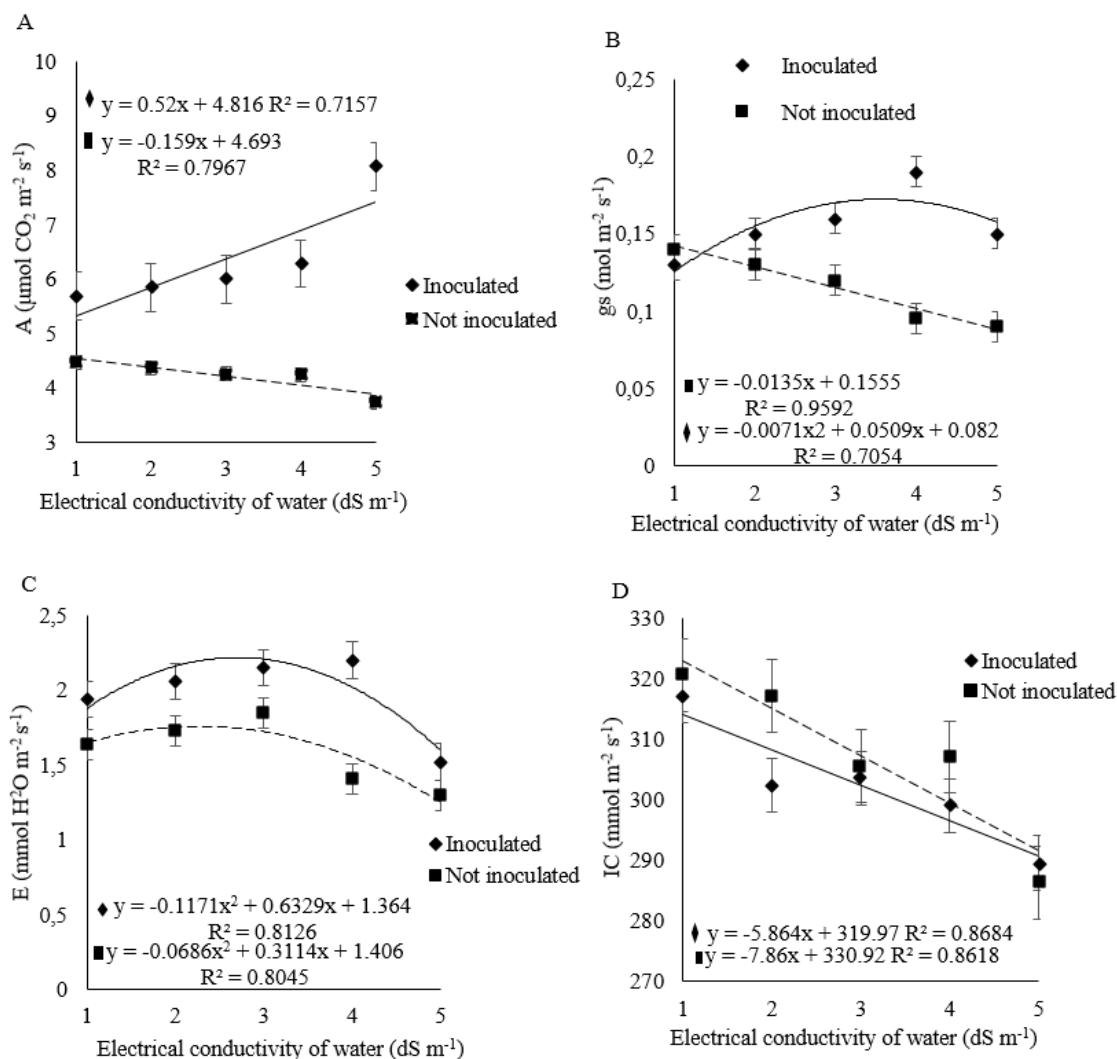
Figure 1. A: Photosynthesis (A), g_s : stomatal conductance (B), E: Transpiration (C) and IC: Internal concentration of \text{CO}_2 (D), of inoculated and non-inoculated peanuts, submitted to different levels of salinity.
