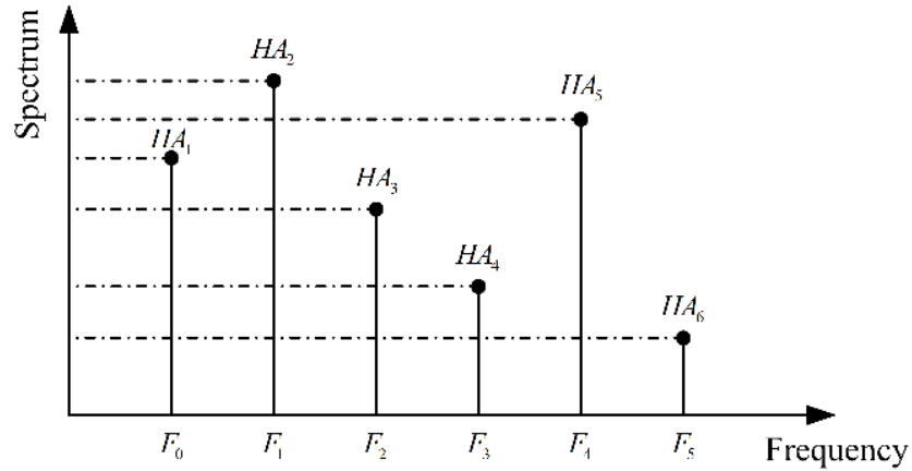
Figure 3.11: Harmonic amplitude difference.
