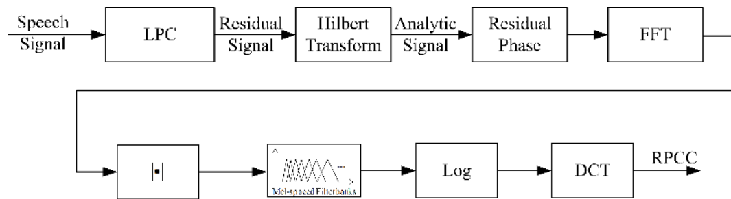
Figure 3.15: Calculation of residual phase cepstrum coefficients.
