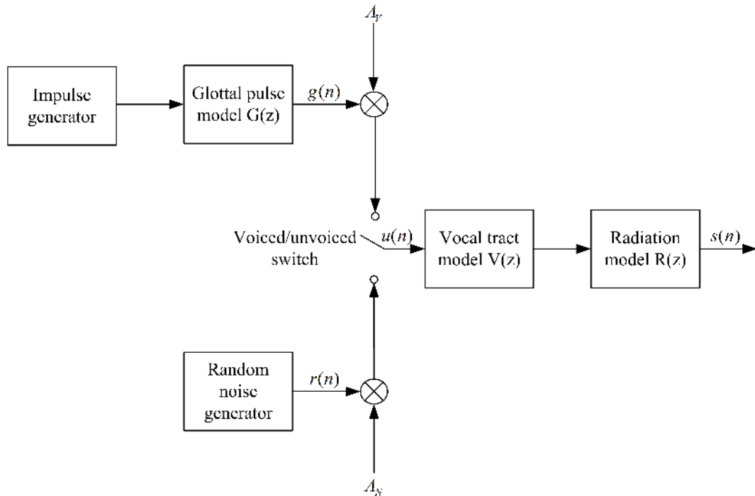
Figure 3.4: Acoustic model for speech production.
