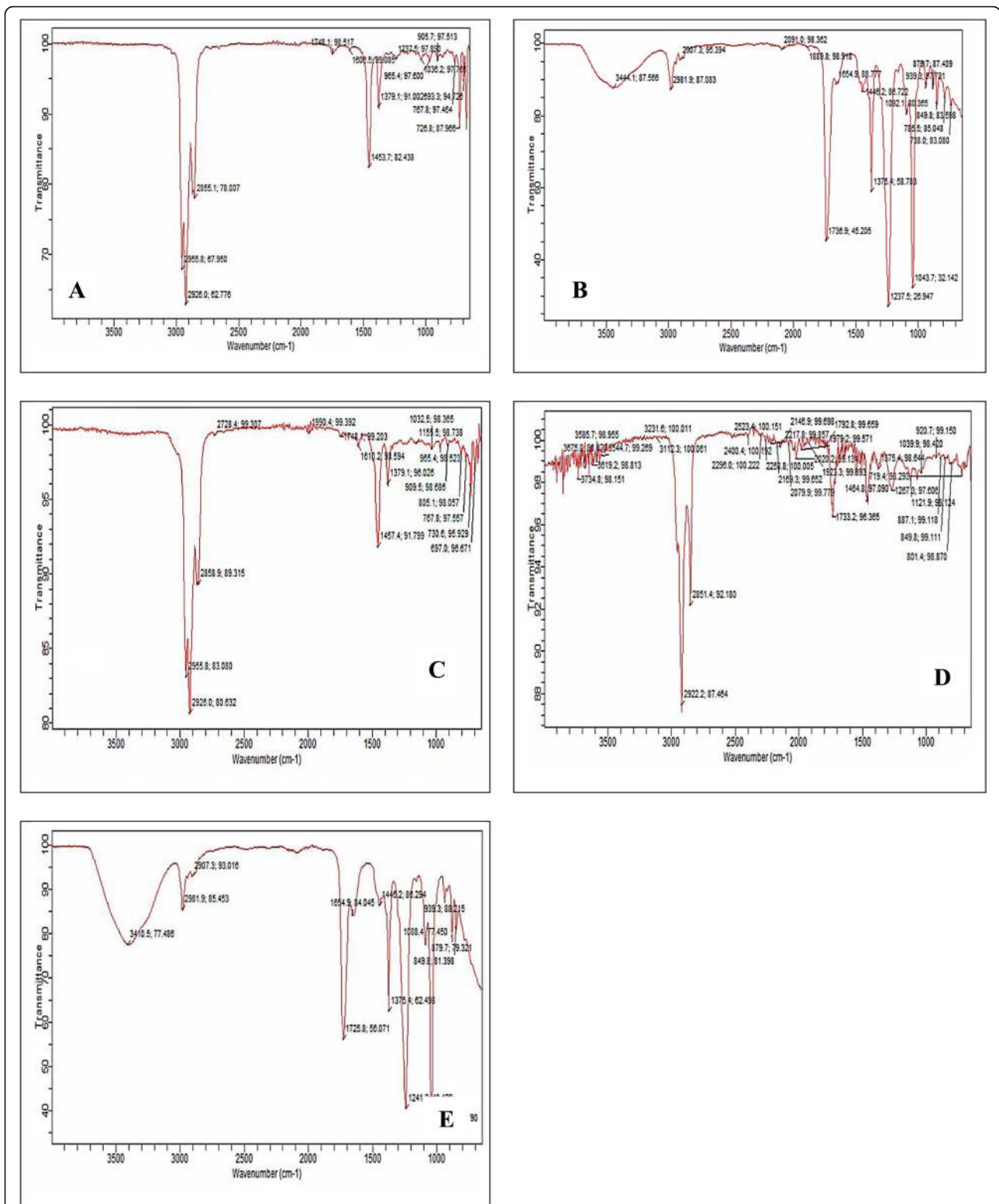
Fig. 5 FT-IR spectra of a Petroleum ether extract of A. occidentale . b Ethylacetate extract of A. occidentale . c n -hexane extract of P. guajava . d Petroleum ether extract of T. catappa . e Ethylacetate extract of T. catappa
