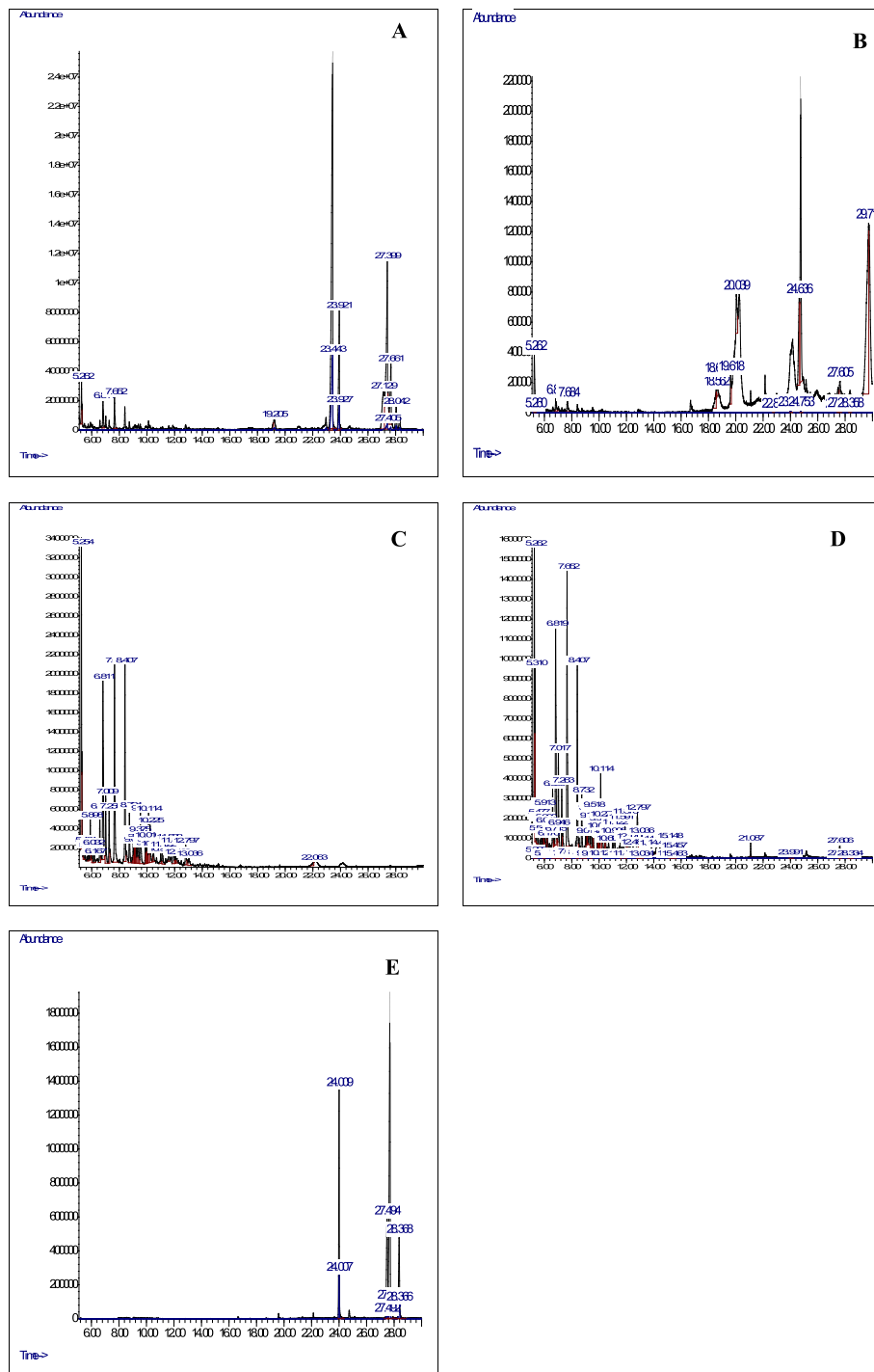
Fig. 4 GC-MS chromatograms: a Petroleum ether extract of A. occidentale . b Ethylacetate extract of A. occidentale . c n -hexane extract of P. guajava . d Petroleum ether extract of T. catappa . e Ethylacetate extract of T. catappa
