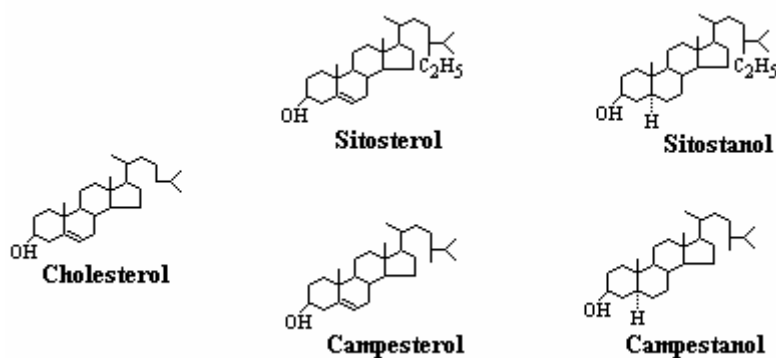
Fig 1. Chemical structures of cholesterol and some phytosterols (Gilbert et al., 2005).
