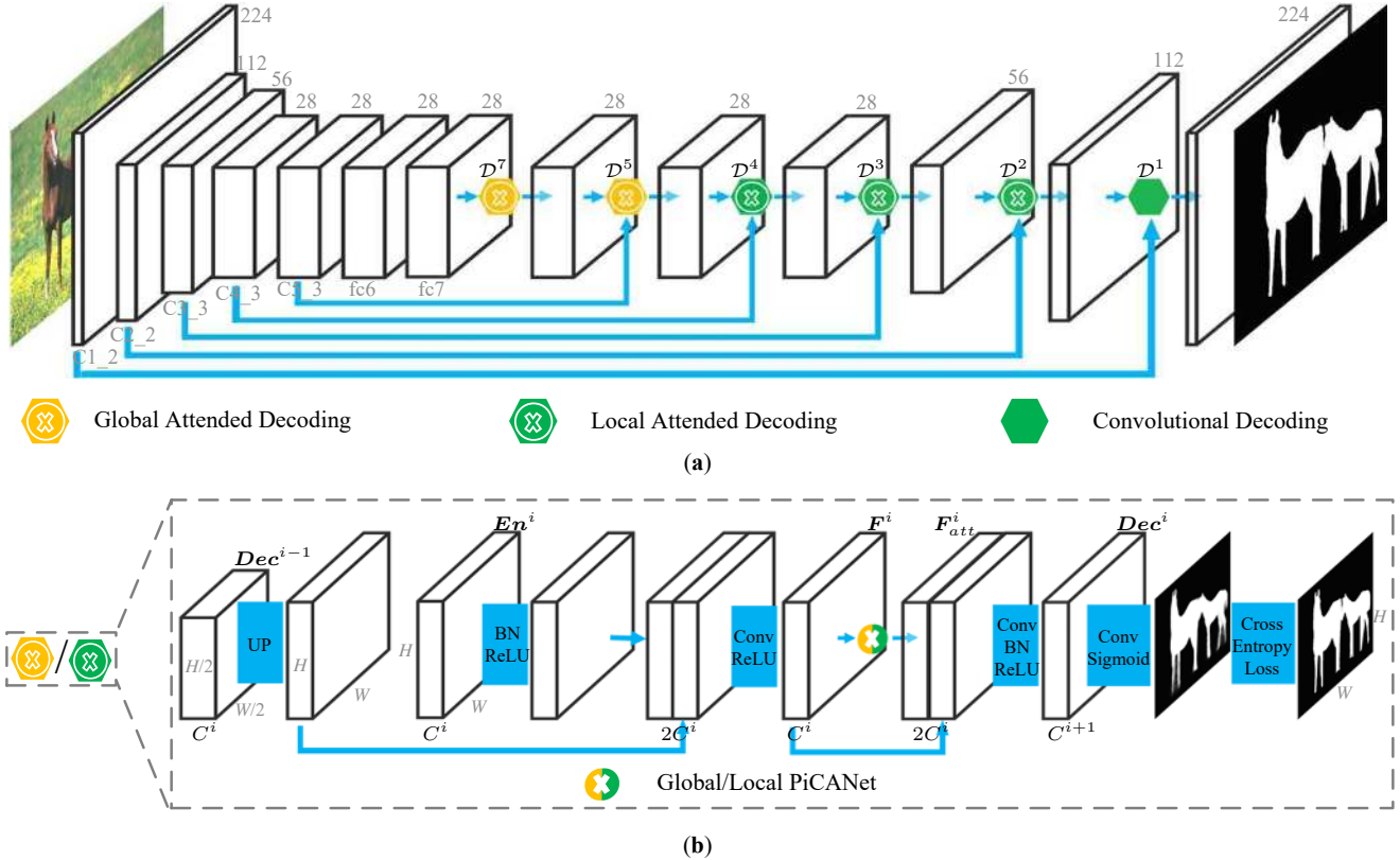
Figure 3. (a) Architecture of our saliency network with the VGG 16-layer backbone. We only show the skip-connected encoder layers of the VGG network. “C” means “convolution” while \mathcal{D}^* indicates a decoding module. The spatial sizes are marked over the cuboids which represent the feature maps. (b) Illustration of an attended decoding module. En^i denotes a convolutional feature map from the encoder network. Dec^i denotes a decoding feature map. F^i denotes a fusion feature map and F_{att}^i denotes its attended contextual feature map. “UP” denotes upsampling. Some important spatial sizes and channel numbers are also marked.
