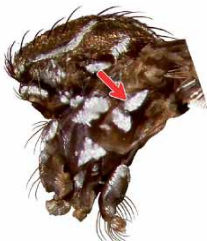
FIGURE 130. Aedes (Stegomyia) aegypti .
