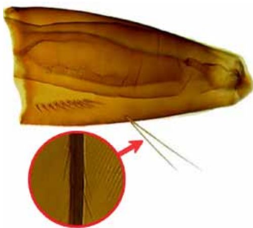
FIGURE 36. Aedes (Stegomyia) africanus .
