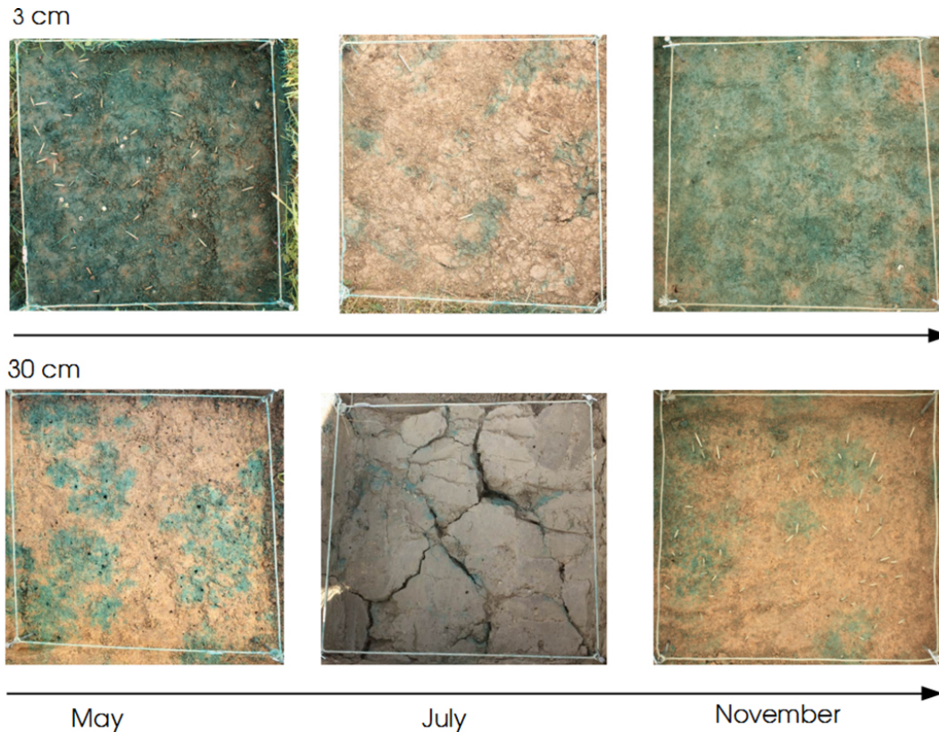
Figure 4. Emergent structures in the Wollefsbach catchment for the sampling dates (plot size is 1\text{ m}^2 ). In May macropore flow through earthworm burrows dominates infiltration, while in July clearly visible soil cracks occur. In contrast, a more homogenous infiltration pattern is visible in November, especially at 3 cm depth.
