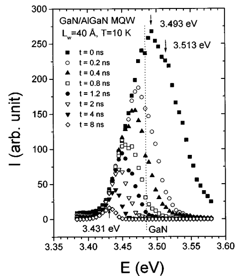
FIG. 2. Low-temperature (10 K) time-resolved photoluminescence spectra of the main emission line in the 40 Å well GaN/Al x Ga 1-x N MQW sample. The dotted line indicates the position of the excitonic transition peak in GaN epilayers grown under similar conditions. Experimental conditions are the same as those in Fig. 1.
