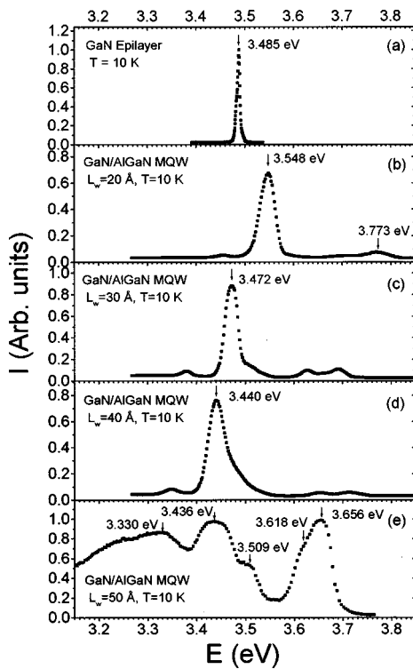
FIG. 1. Low-temperature (10 K) cw PL spectra of nominally undoped GaN/Al x Ga 1-x N MQW samples with well thickness (b) L_w=20 Å, (c) 30 Å, (d) 40 Å, (e) 50 Å, and (a) GaN epilayer grown under identical conditions as the MQW samples, measured at the same experimental conditions.
