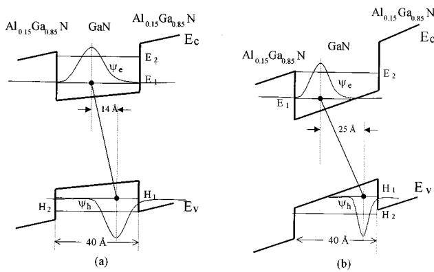
FIG. 4. Schematic energy band diagrams of the GaN/Al 0.15 Ga 0.85 N MQW sample (a) with the piezoelectric field under the influence of screening by photoexcited carriers (or t_d=0 ) and (b) the original piezoelectric field in the absence of carrier screening (or after long delay times).
