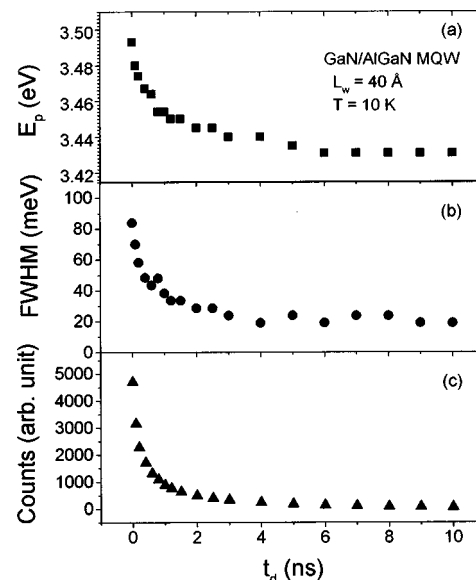
FIG. 3. (a) Peak position E_p , (b) the full width at half maximum (FWHM), and (c) total counts of the main emission line in the 40 Å well GaN/Al x Ga 1-x N MQW sample as functions of delay time measured at T=10 K.
