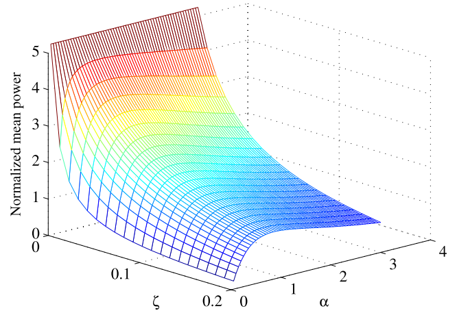
Figure 2. The normalized mean power of a harvester without an inductor as a function of \alpha and \zeta , \kappa = 0.6 .
