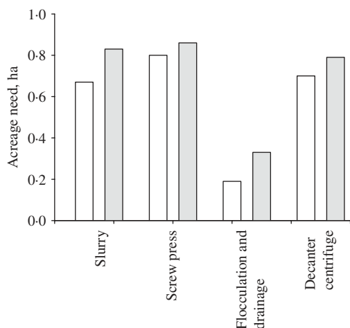
Fig. 3. The field area needed for spreading 30 t of slurry or the liquid manure fraction obtained from separating 30 t of slurry to fulfil winter wheat requirements for available nitrogen (adjusted to MFE). Untreated (□) and acidified fractions (■).
