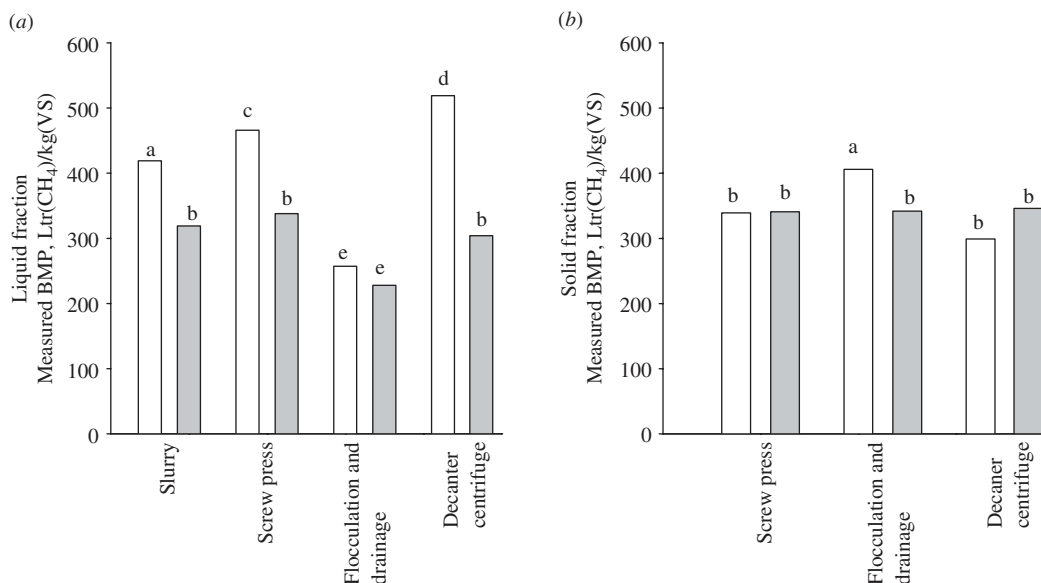
Fig. 2. Biogas production potential: (a) measured BMP of slurry and liquid fraction and (b) measured BMP of solid fraction. Bars with different letters are significantly different ( P < 0.05 ). Untreated (□) and acidified fractions (■).
