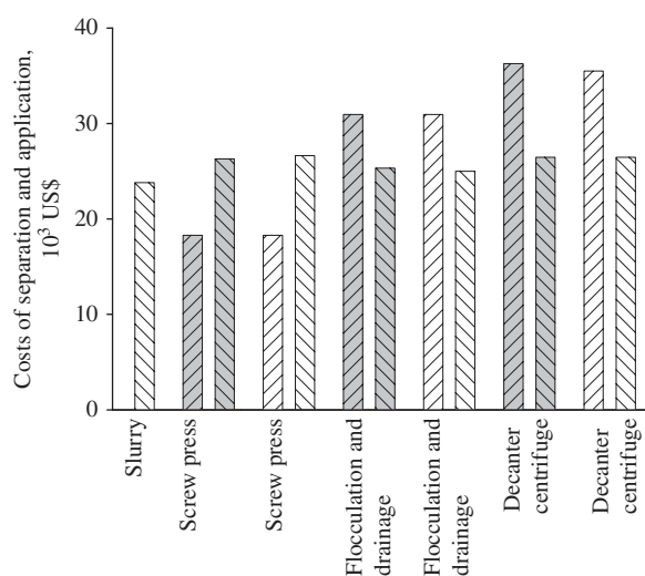
Fig. 6. Total costs of separation and application in US$. Separation and untreated (▨), separation and acidified (▧), application and untreated (▩) and application and acidified (▪).
