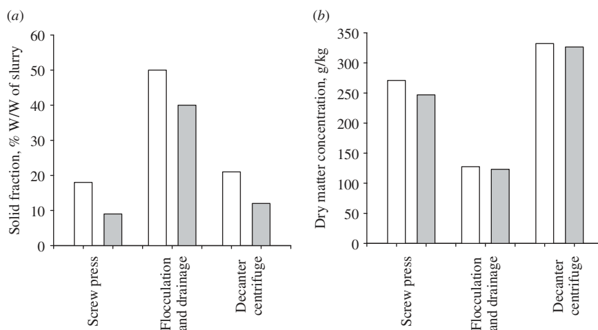
Fig. 1. Separation of slurry as affected by separation technology and the acidification of slurry: (a) the amount of solid manure fraction as a fraction of slurry treated and (b) DM concentration in solid manure fraction. Untreated (□) and acidified fractions (■).
