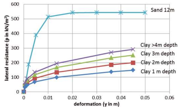
Fig. 22. (Color) p - y curves at different depths for clay and sand for pile diameter of 0.18 m according to API (1984) as used in Bijmagne and Luger (2000) (determined for a 11.5-m-thick saturated clay with c_u = 30 kN/m 2 ; \gamma' = 16 kN/m 3 ; empirical constant J = 0.25 ; and \epsilon_{50} = 0.01 and 0.5 m sand with \varphi' = 30^\circ ; \gamma' = 19.8 kN/m 3 ; K_0 = 0.5 ; factor for static loads A = 0.9 ; initial modulus of subgrade reaction k = 8,145 kN/m 3 ; and q_c = 13.5 MPa)
