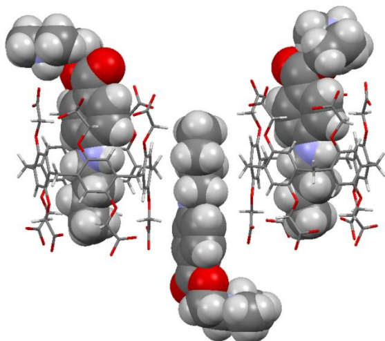
Figure 7. X-Ray structure of 4a -tetracaine
