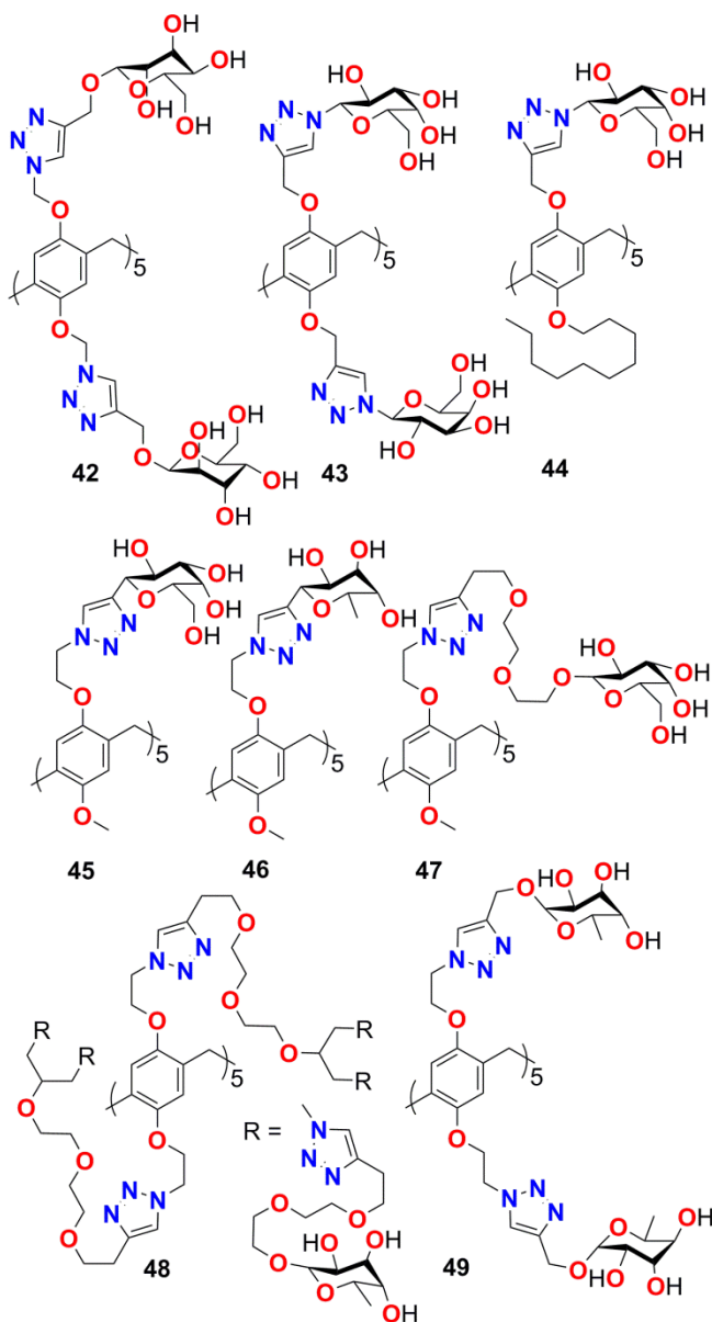
Figure 10. Pillar[n]arene glycoclusters 42 – 49 .
