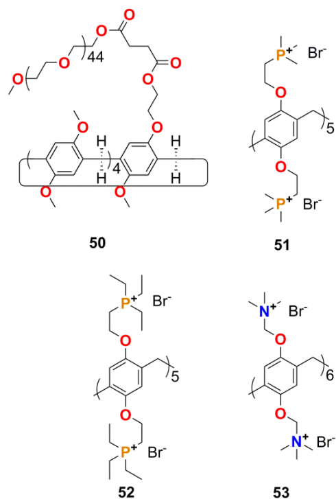
Figure 11. Therapeutic pillar[n]arenes 50 – 53 .
